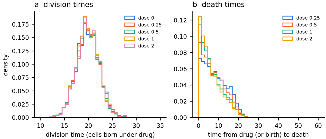
Figure S1. Single-cell timing distributions underlying Figure 4c. (a) Division times of cells born under drug and (b) times from drug start (or from birth, for cells born under drug) to death, per dose.
