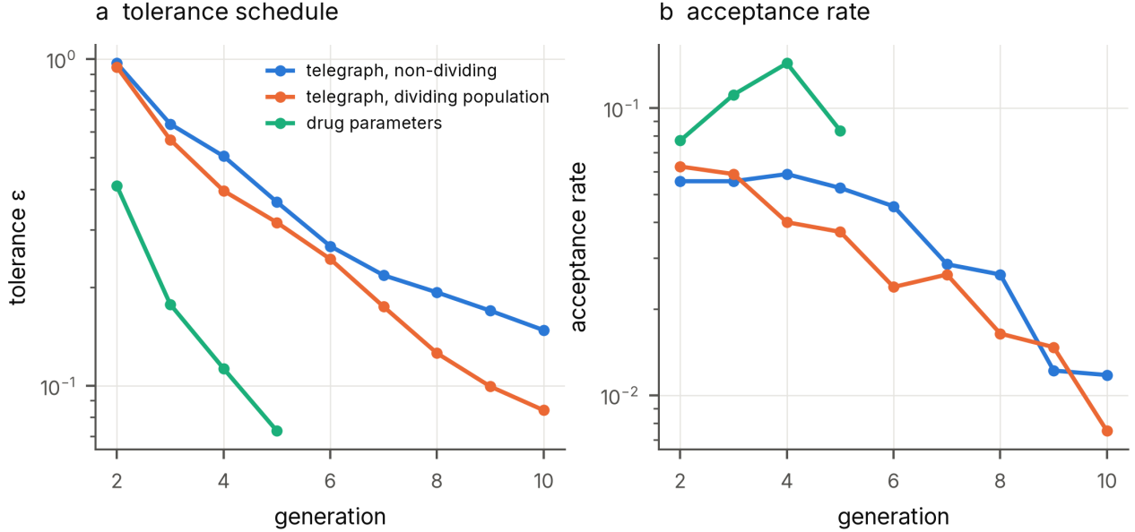
77 78 Supplementary Fig. 2 | ABC-SMC diagnostics. a , Tolerance and b , acceptance rate per generation for the 79 three runs of Fig. 6.
