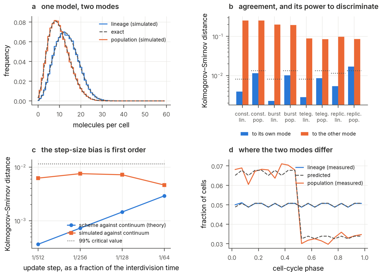
Supplementary Fig. 6 | The population and lineage layers against exact solutions. a , Simulated and exact stationary distributions for constitutive production with a memoryless interdivision time, in single-lineage and population-snapshot mode. b , Kolmogorov-Smirnov distance to the exact law of the matching mode, and to the exact law of the other mode, for every model; the dotted line is the 99% critical value at the sample size used. c , Kolmogorov-Smirnov distance against the update step, showing the discretisation of the interdivision time vanishing. d , Measured and predicted distribution of cell-cycle phase, for the model with gene replication. Along a lineage the phase is uniform. In the population it is the two-level step that a deterministic cycle produces: the snapshot is taken half a cycle after a whole number of generations, and the cells younger than that are the ones whose ancestors have divided once more, so they are twice as numerous. The position of the step is set by when the snapshot is taken and has nothing to do with the replication point, which is also at mid-cycle. The prediction is obtained by iterating the age map of the scheme from the founder ages used.
