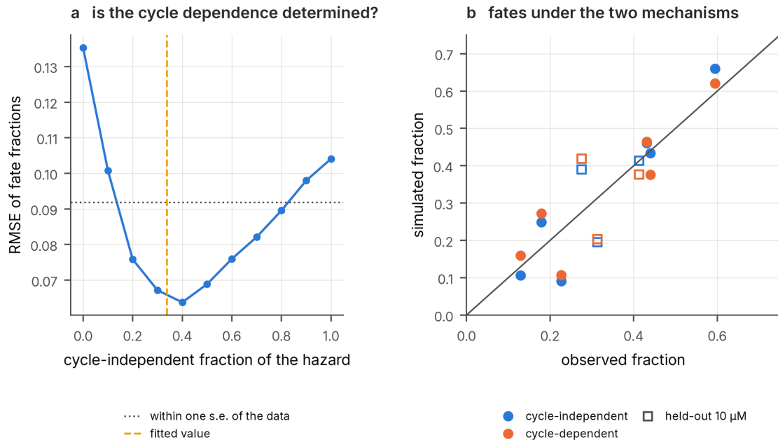
144 145 Supplementary Fig. 4 | Cell-cycle-dependent killing tested against the fate data. a , Root-mean-square 146 error of the fate fractions at the training concentrations as the cycle-independent fraction \beta of the death hazard is 147 moved from 0 (killing confined to the replication window) to 1 (cycle-independent), with the remaining parameters 148 held at the cycle-dependent fit; dotted line, one binomial standard error of the measurement above the best fit; 149 dashed line, the fitted value. b , Simulated against observed fate fractions at all three concentrations for the 150 cycle-independent and the cycle-dependent fit (squares, the held-out 10 \mu M condition; line, equality).
