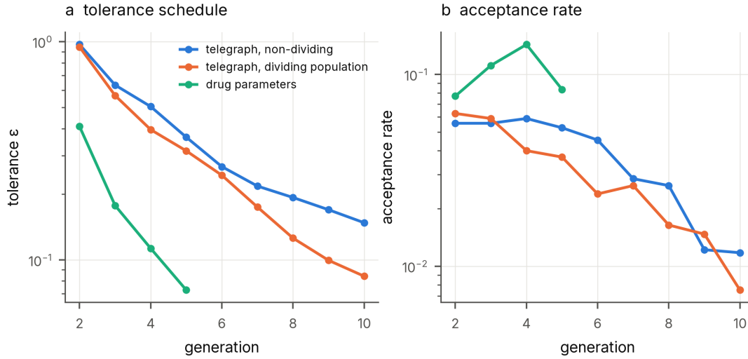
79 Supplementary Fig. 2 | ABC-SMC diagnostics. a , Tolerance and b , acceptance rate per generation for the 80 three runs of Fig. 6.
