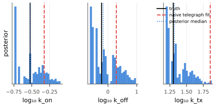
b dividing population: division-aware ABC vs naive fit
