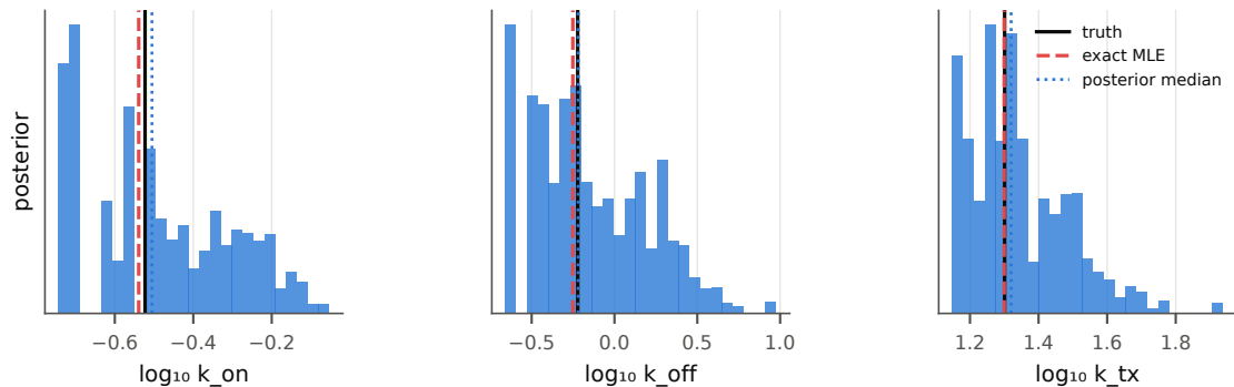
a non-dividing cells: ABC vs exact MLE
