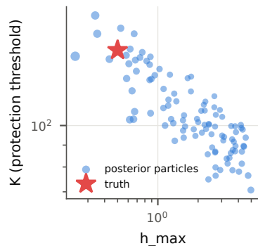
c drug parameters from kill curve + sister fates
