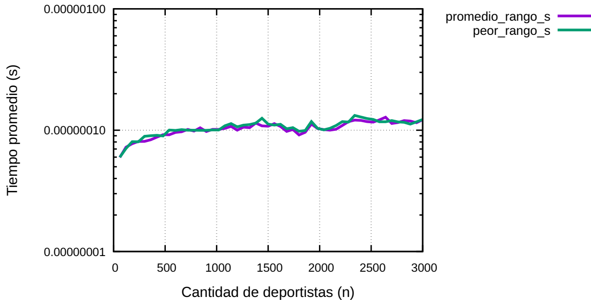
Binary range search benchmark
