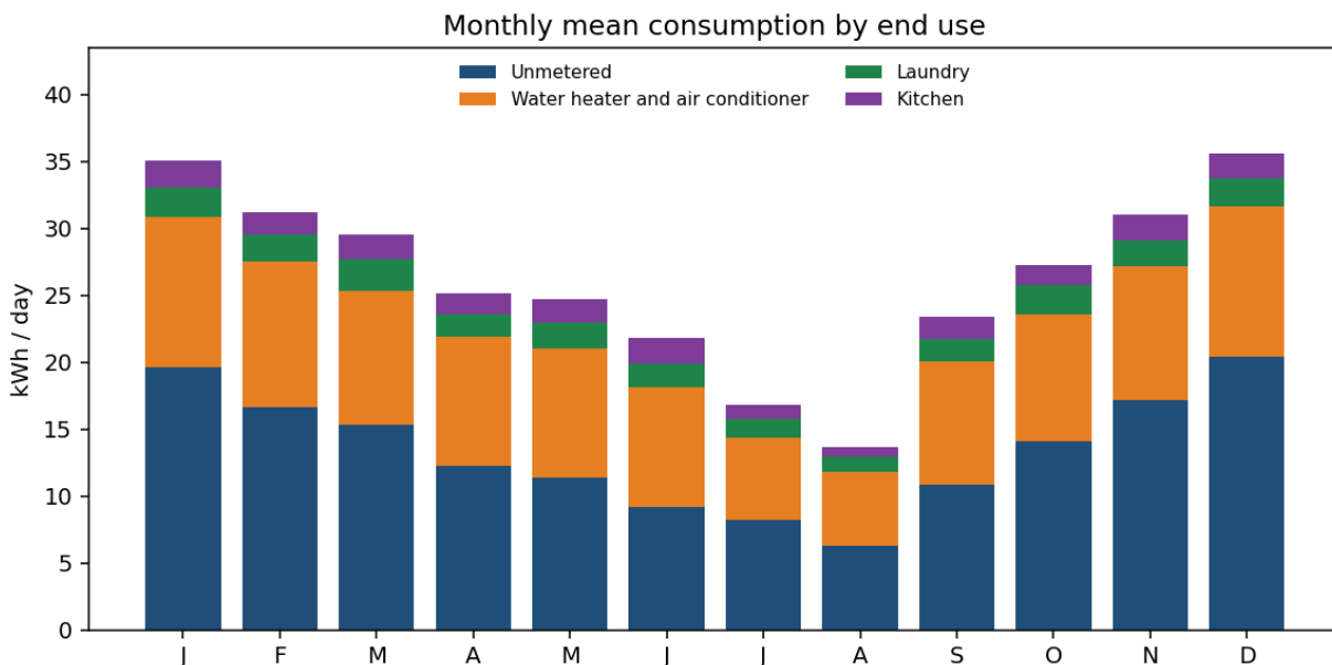
Figure 3: Monthly mean consumption by end use. Sub-meter 3 is the circuit the dataset labels as the water heater and air conditioner. It falls from winter into summer, which is the water heater’s direction.
