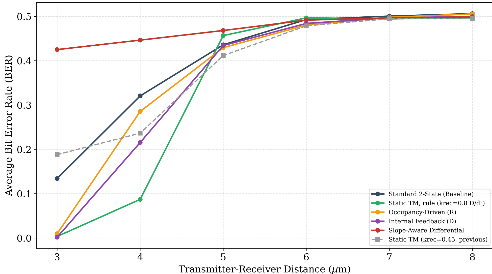
BER versus Distance under 3D Fickian Diffusion Channel
