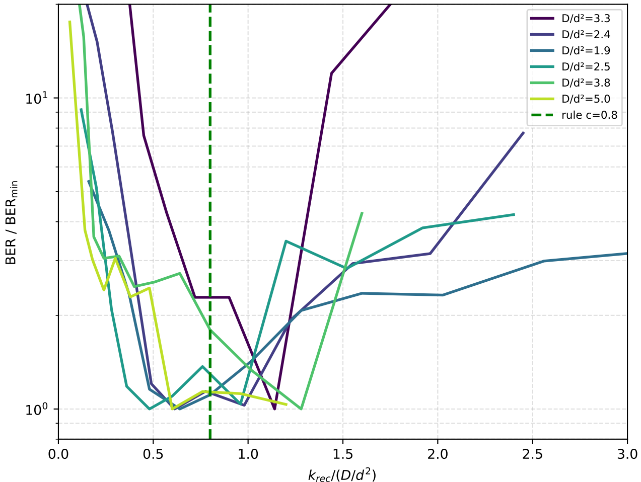
Collapse test: minima cluster near the rule
