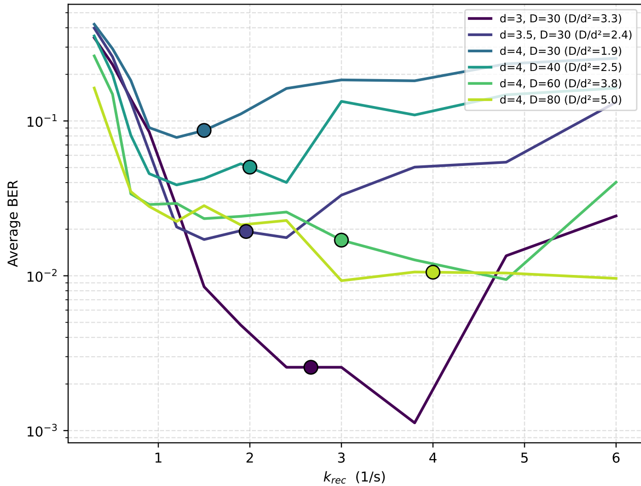
BER valley vs k_{rec} (markers = rule 0.8D/d^2 )
