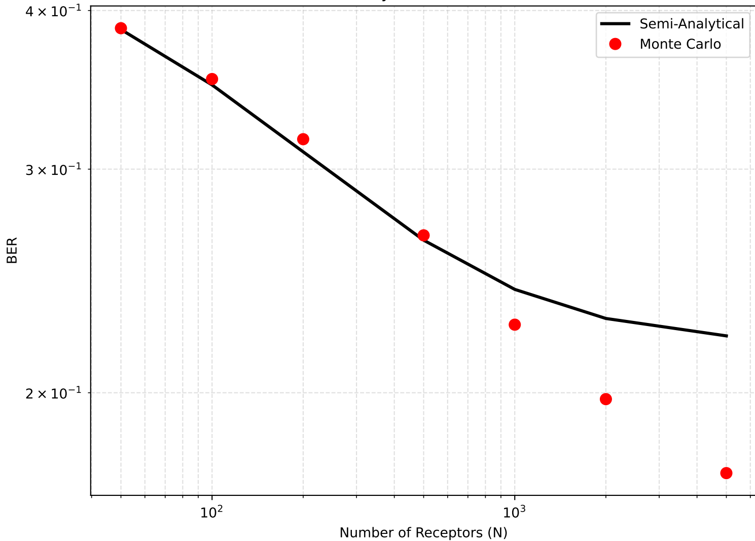
Semi-Analytical BER Validation
