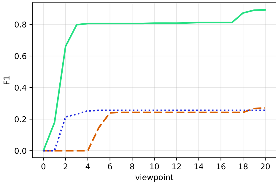
(RH-NBV) Effect of the candidate budget (coffee mug & panels3)
