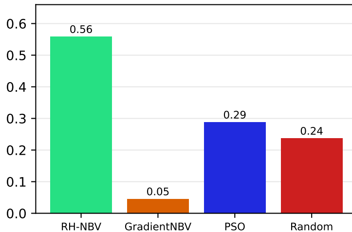
Move success (%)
