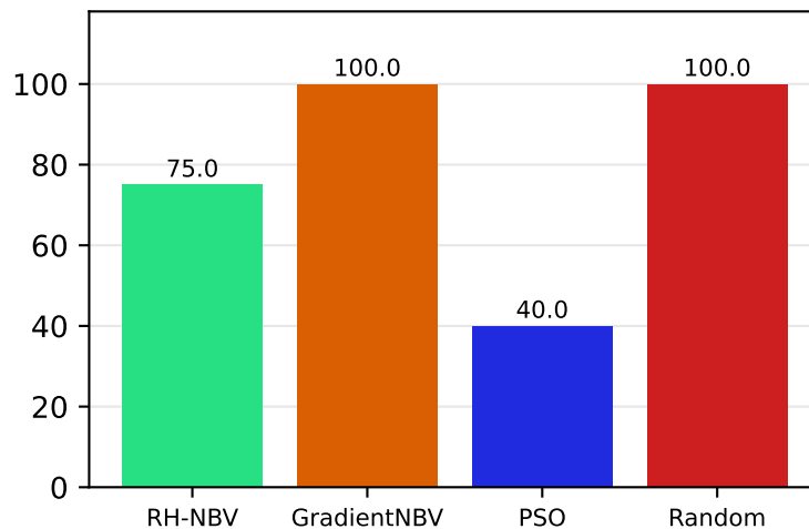
Move success (%)
