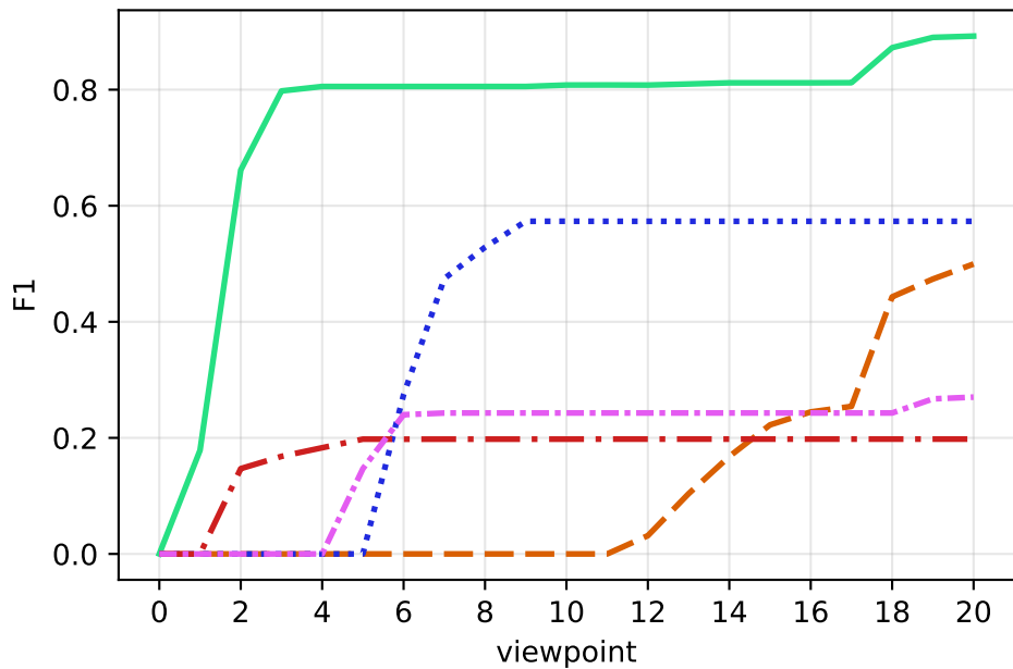
(RH-NBV) Effect of the planning horizon (coffee mug & panels3)
