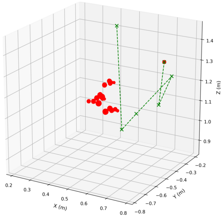
(b) PSO, 5/20 motions executed
