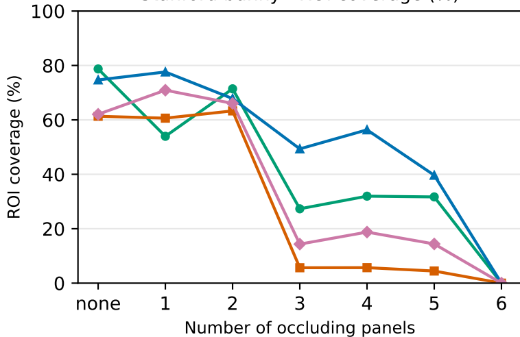
Stanford bunny - ROI coverage (%)
