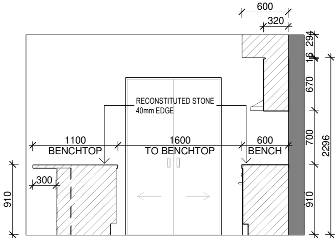
ELEVATION - KA KITCHEN ELEVATIONS
