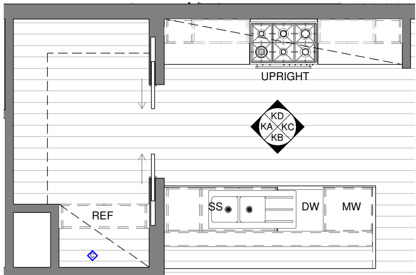
KITCHEN PLAN SCALE 1 : 50
