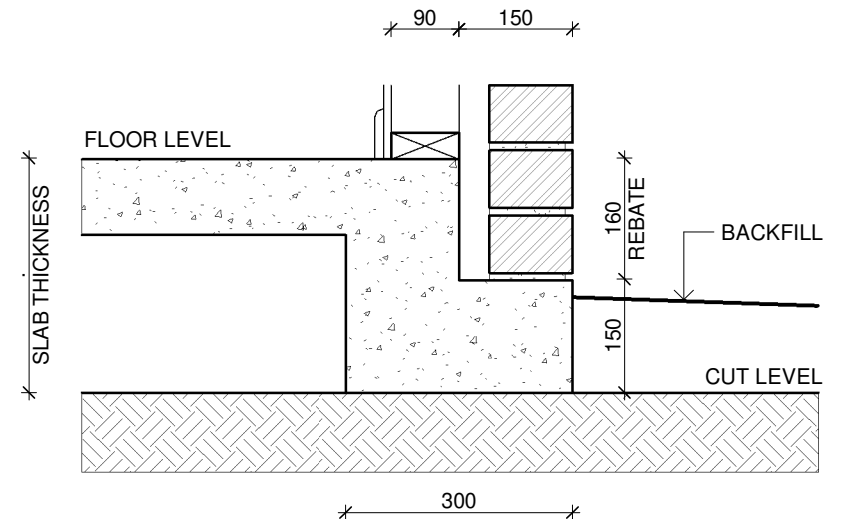
2 BRICK REBATE - TYPICAL 1 : 10
