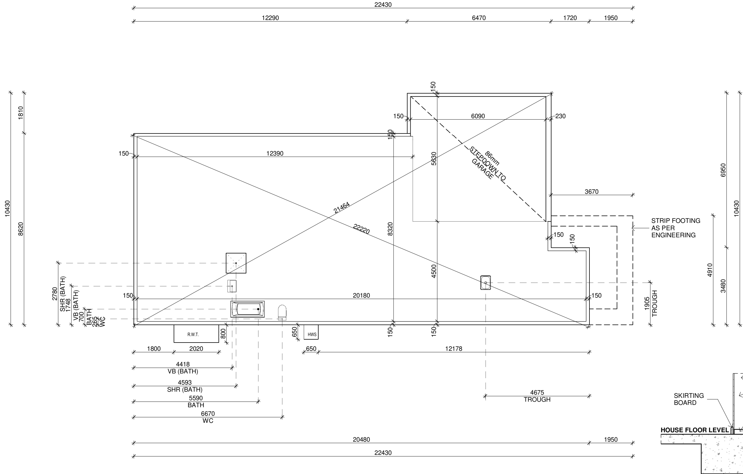
SLAB LAYOUT SCALE 1 : 100
