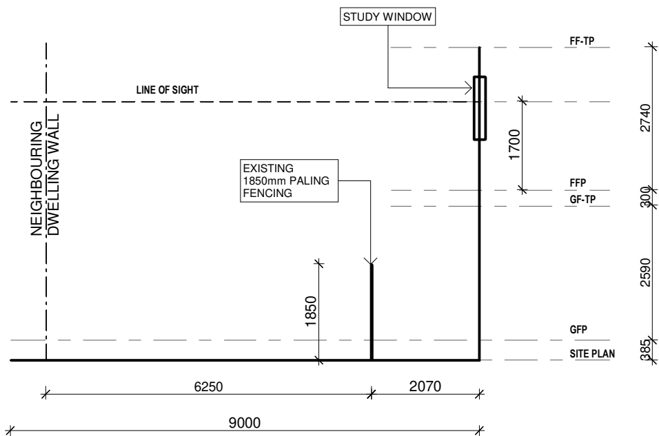
OVERLOOKING DIAGRAM 1 SCALE 1 : 100
