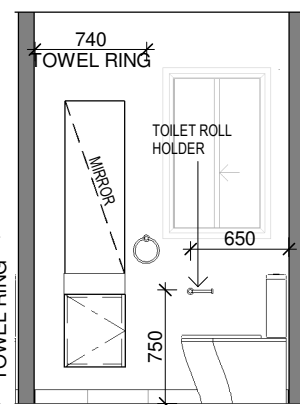
ELEVATION - PD
