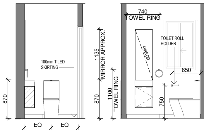
ELEVATION - PC
