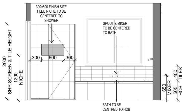
ELEVATION - EA ENSUITE ELEVATIONS
