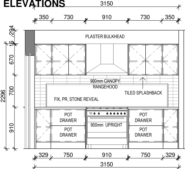
ELEVATION - KD
