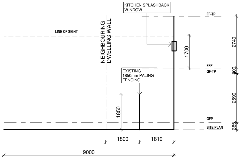
OVERLOOKING DIAGRAM 2 SCALE 1 : 100
