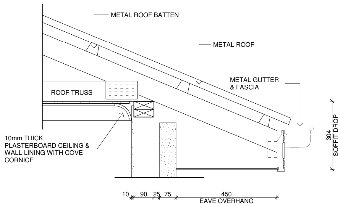
3 450mm EAVE DETAIL 1 : 10
