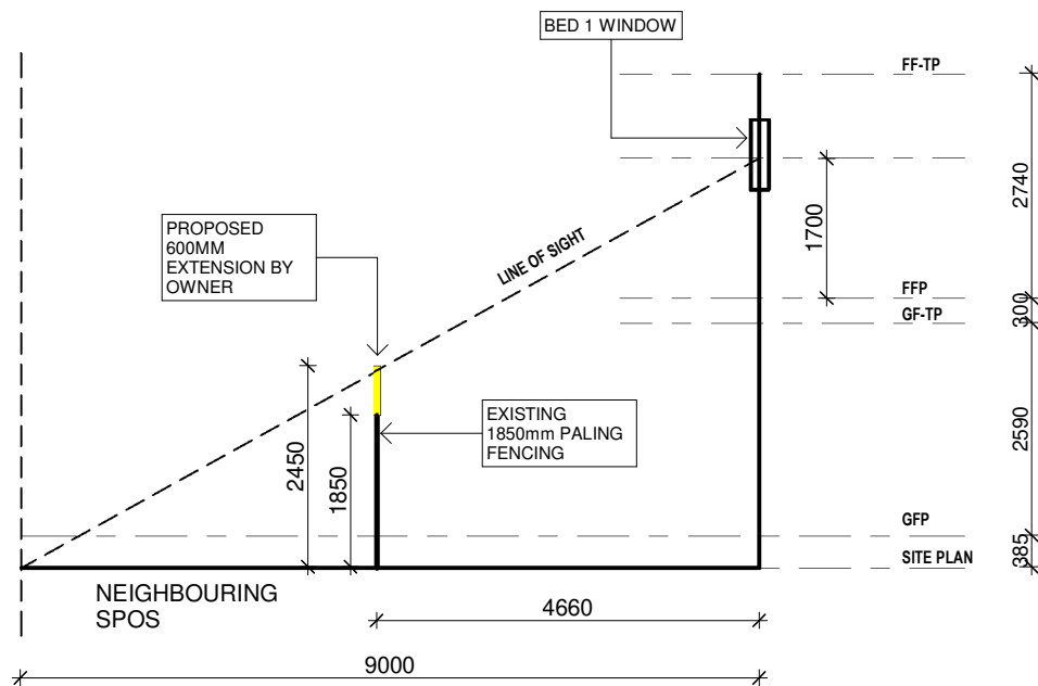
OVERLOOKING DIAGRAM 3 SCALE 1 : 100
