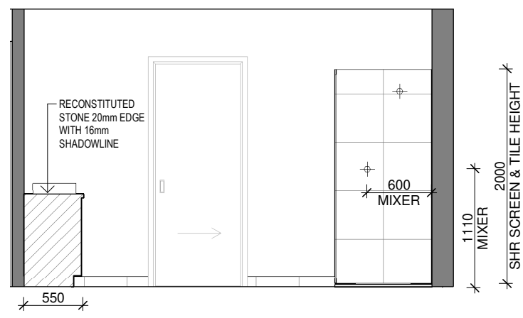
ELEVATION - EB
