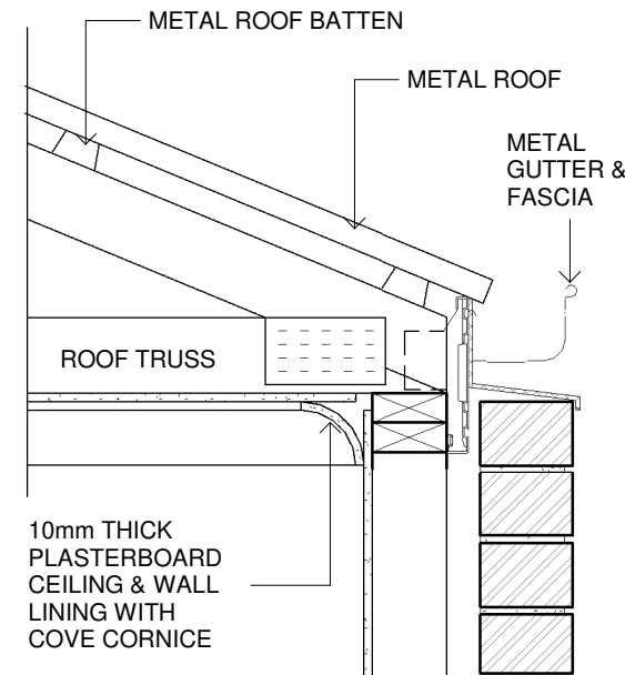
1 GUTTER ON BRICK 1 : 10
