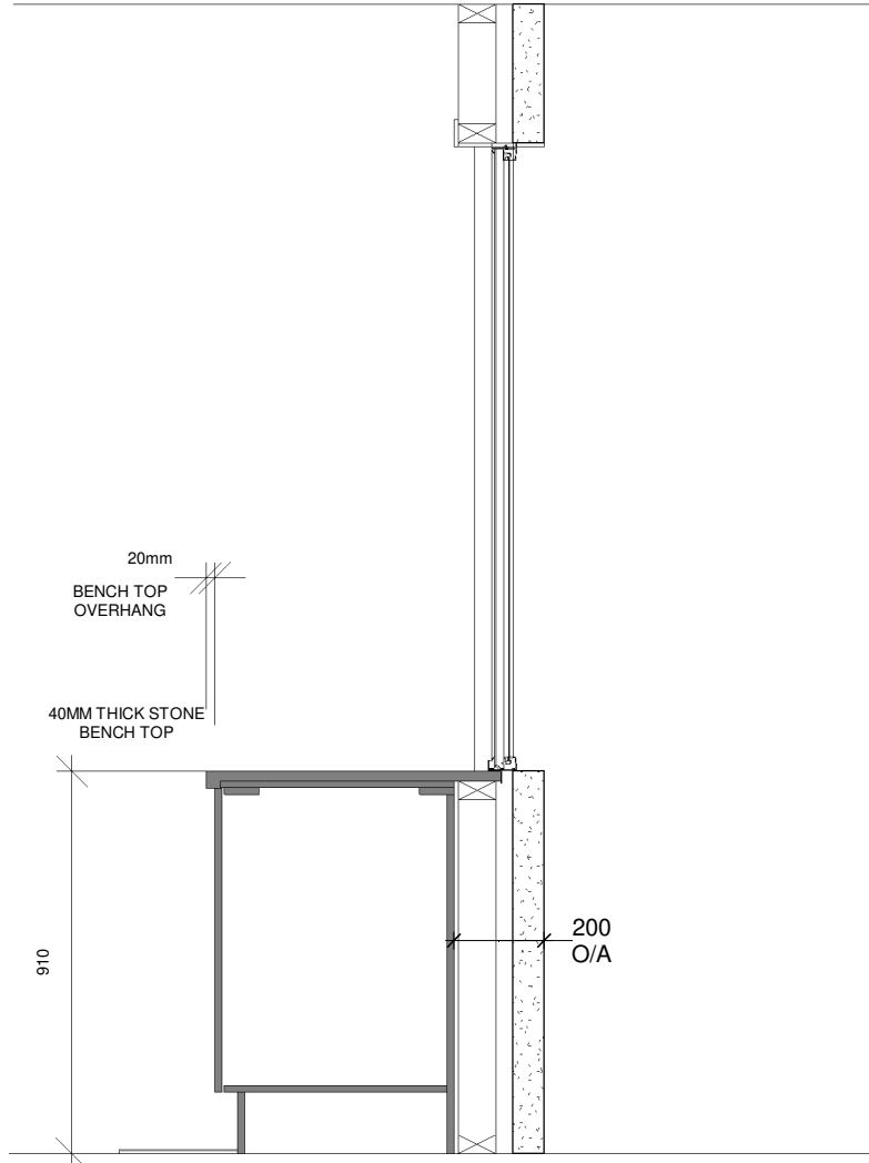
STONE REVEAL DETAIL SCALE 1 : 20
