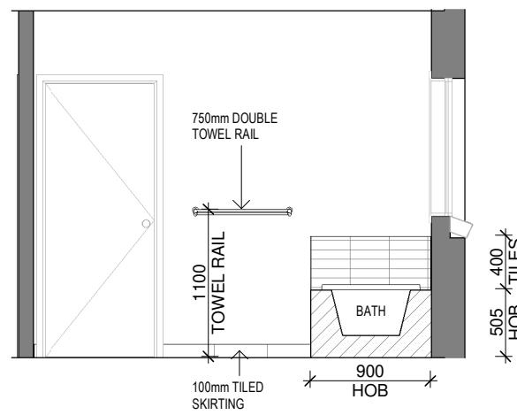
ELEVATION - BC
