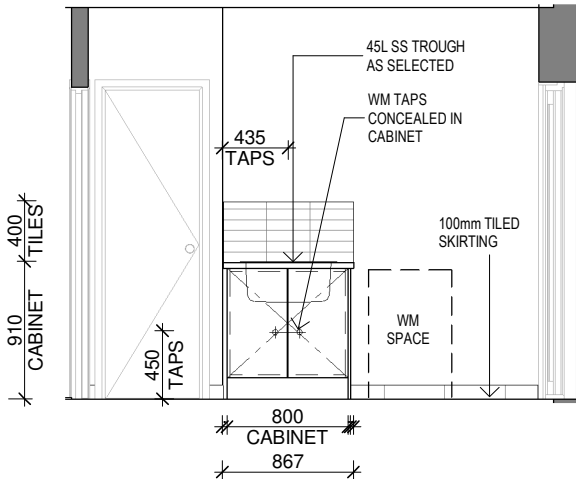
ELEVATION - LC LAUNDRY ELEVATIONS
