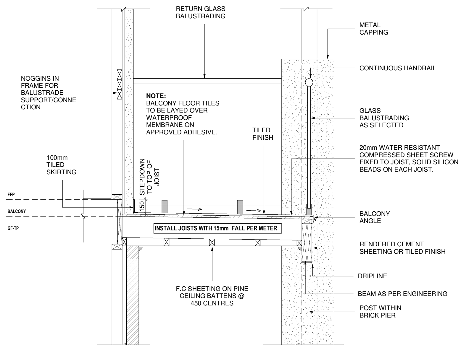
BALCONY DETAIL SCALE 1 : 20
