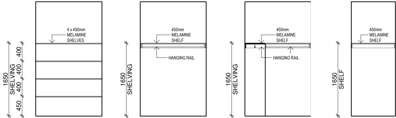
PANTRY / LINEN ROBE TYPICAL INTERNAL ELEVATIONS
