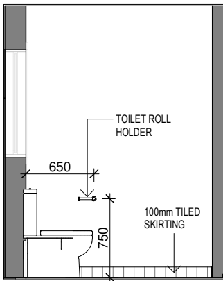
ELEVATION - WA WC ELEVATIONS
