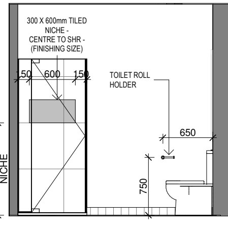
ELEVATION - PC
