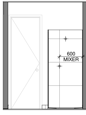
ELEVATION - PB
