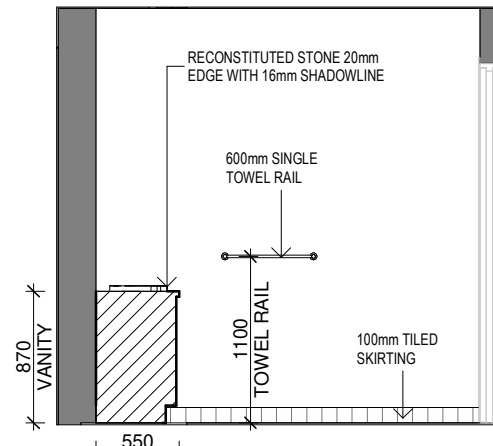
ELEVATION - PA PDR ELEVATIONS
