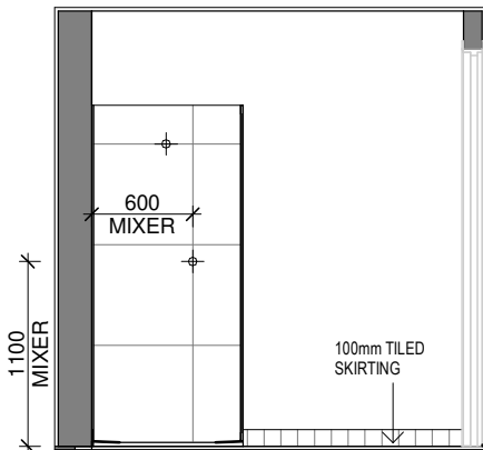
ELEVATION - E3A ENS 3 ELEVATIONS
