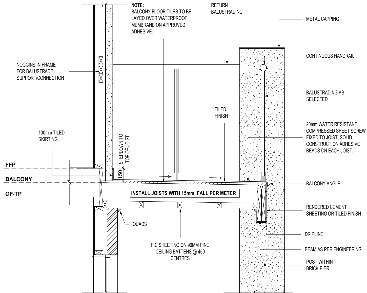
BALCONY 2 DETAIL SCALE 1 : 20
