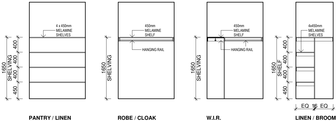
PANTRY / LINEN ROBE / CLOAK W.I.R. LINEN / BROOM TYPICAL INTERNAL ELEVATIONS
