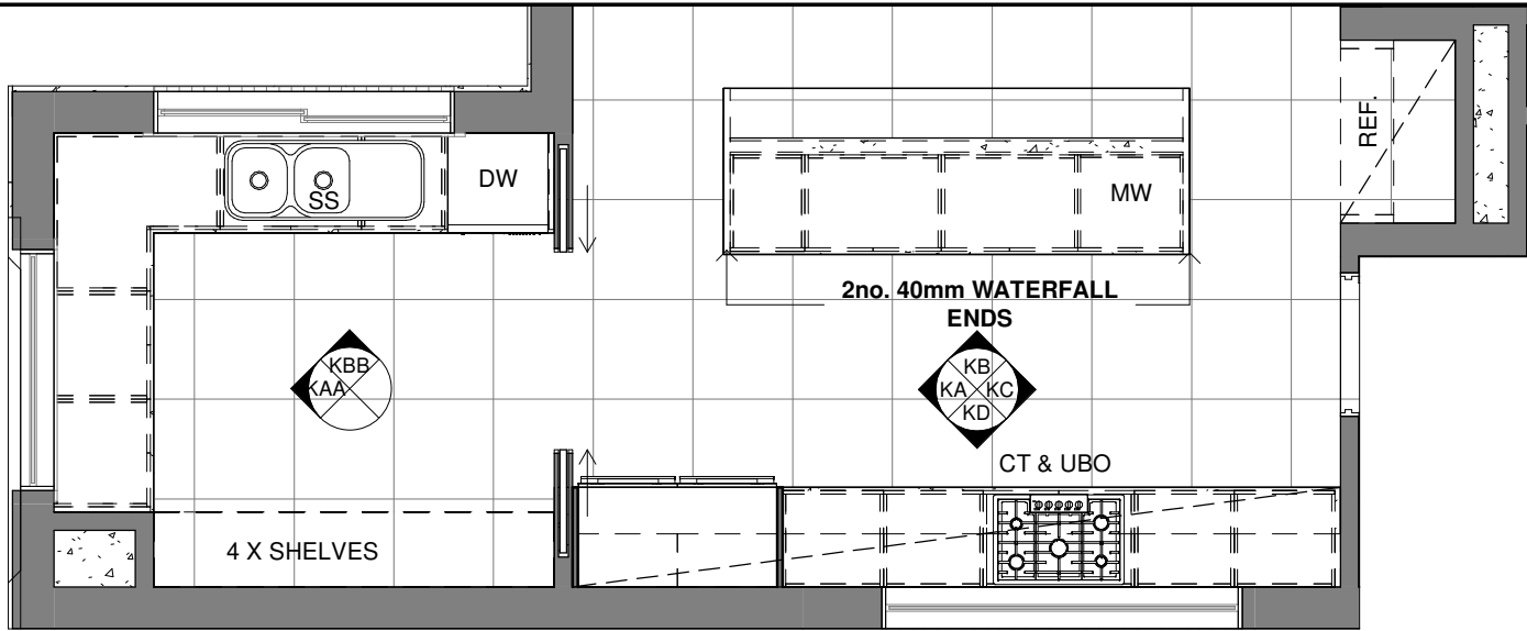
KITCHEN & BUTLERS PLAN SCALE 1 : 50
