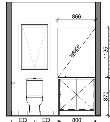
ELEVATION - PD
