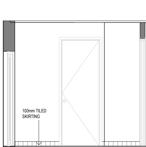
ELEVATION - LA LAUNDRY ELEVATIONS
