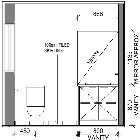
ELEVATION - E2A ENS 2 ELEVATIONS
