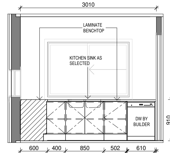
ELEVATION - KBB
