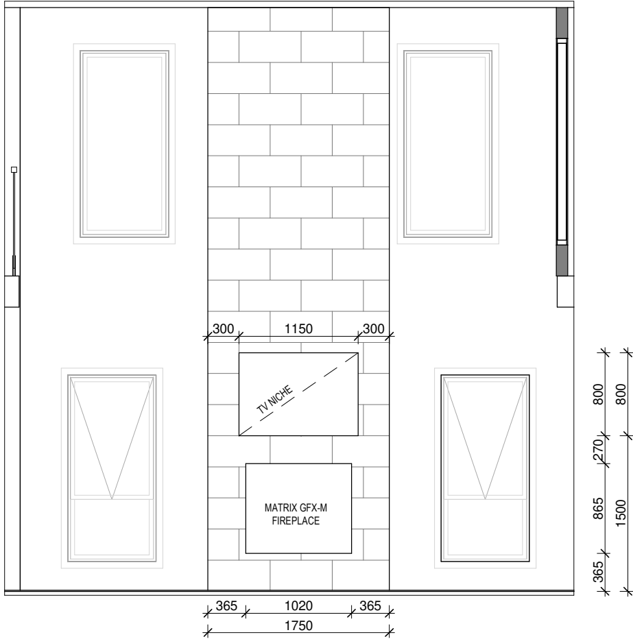
LIVING ROOM FIREPLACE DETAIL - ELEVATION - FB
