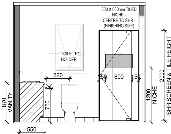
ELEVATION - E4A ENS 4 ELEVATIONS
