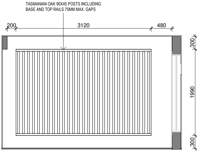
STUDY FEATURE WALL
