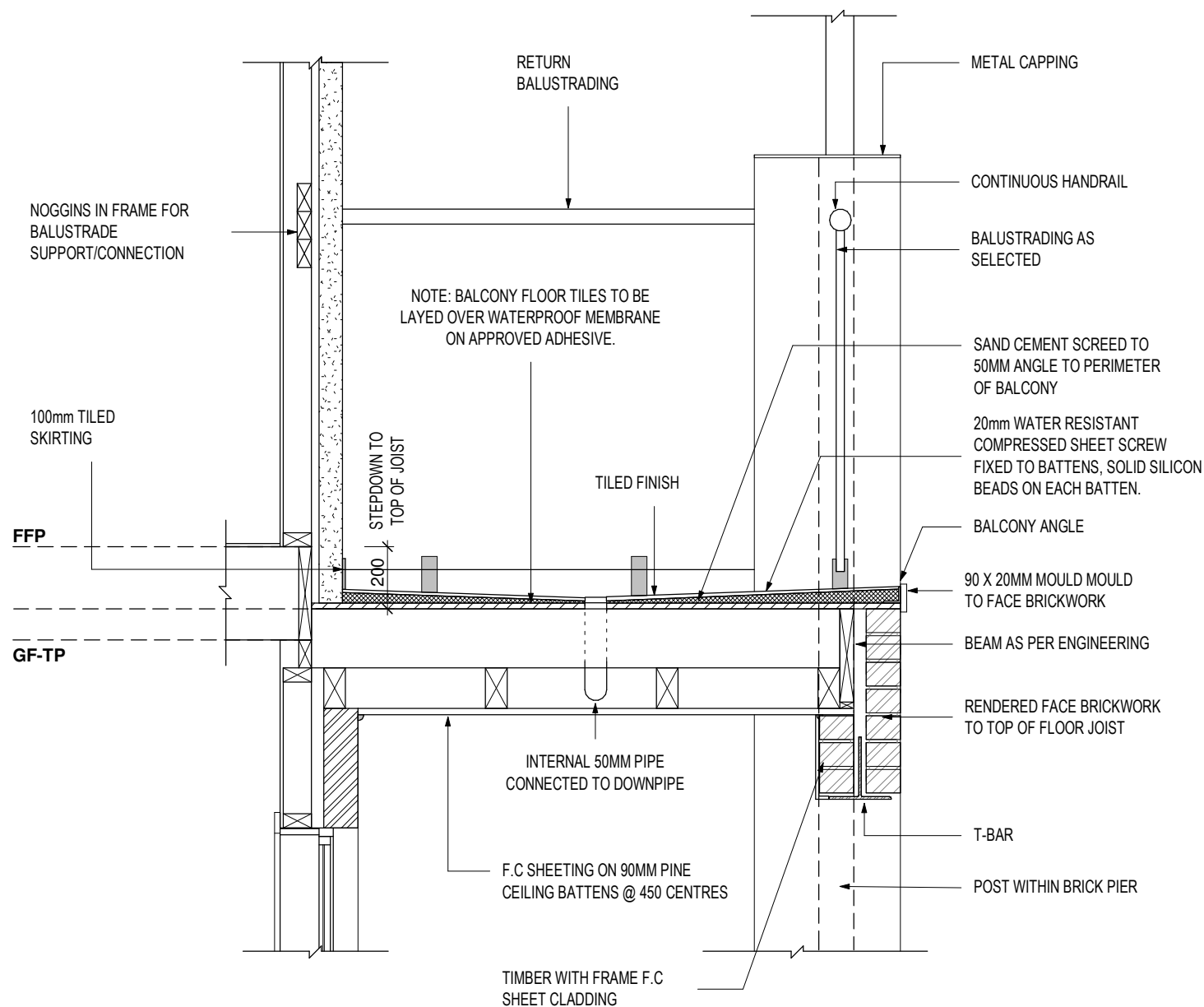
BALCONY 1 DETAIL SCALE 1 : 20
