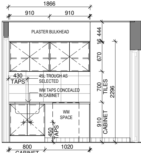
ELEVATION - LC
