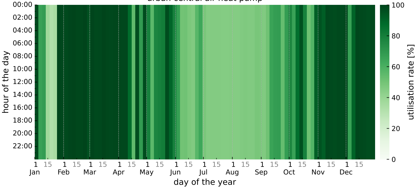
urban central air heat pump
