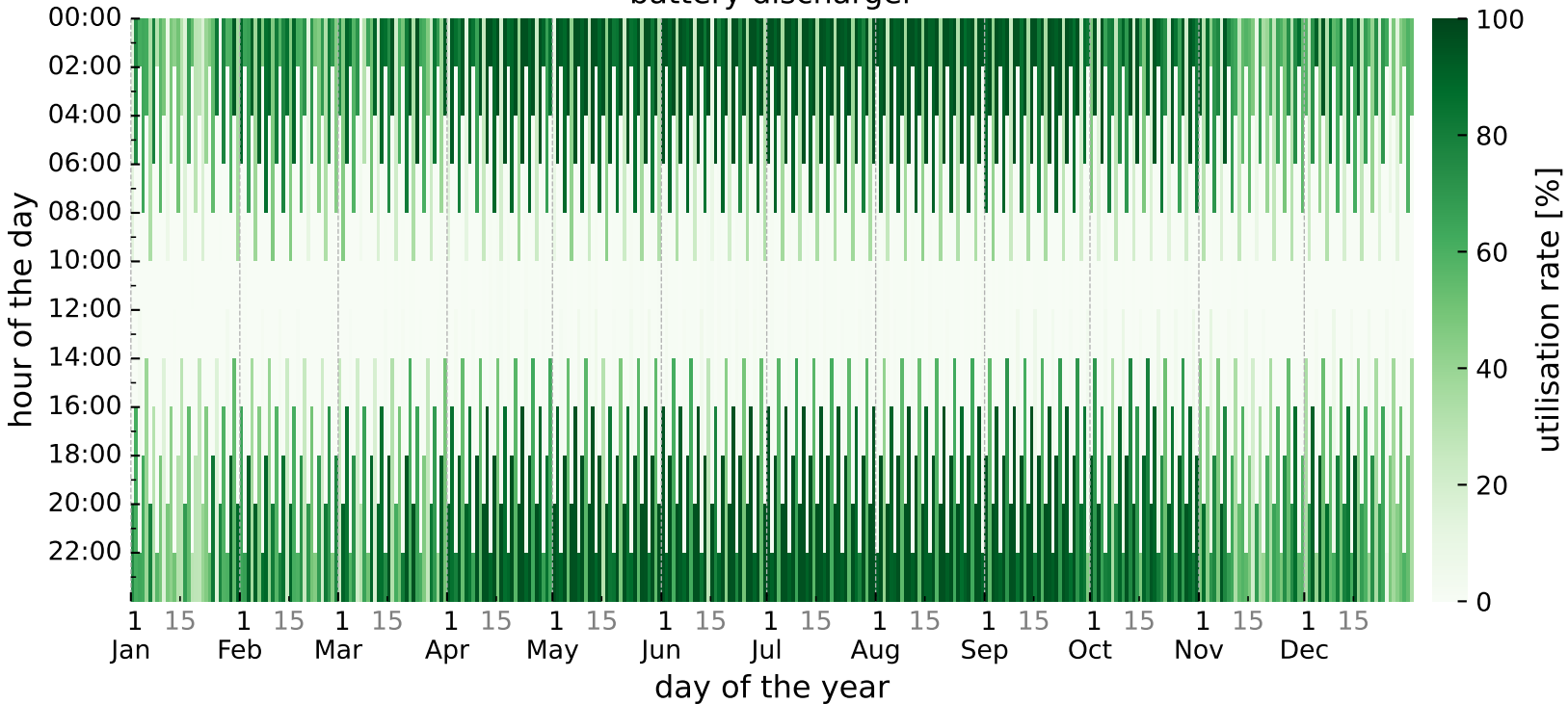
battery discharger
