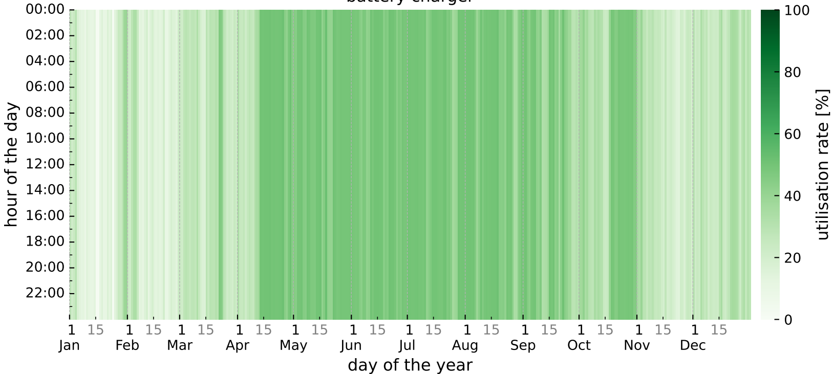
battery charger
