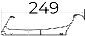
① louvres Profile
