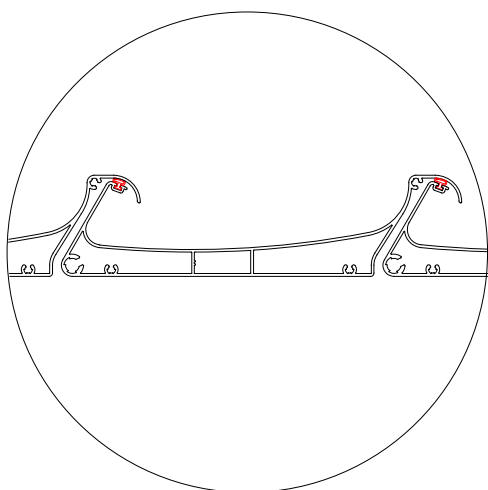
When closed from the panels, it provides sealing thanks to the wicks.
