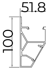
⑥ Profile for RGB and linear Led
