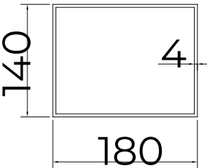
④ Carrier Post Profile
