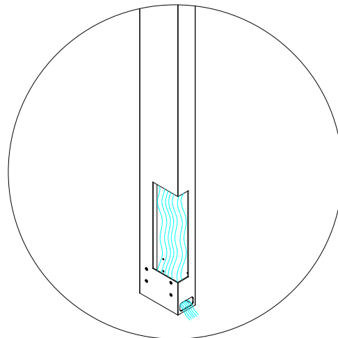
Evacuation of water in the posts
