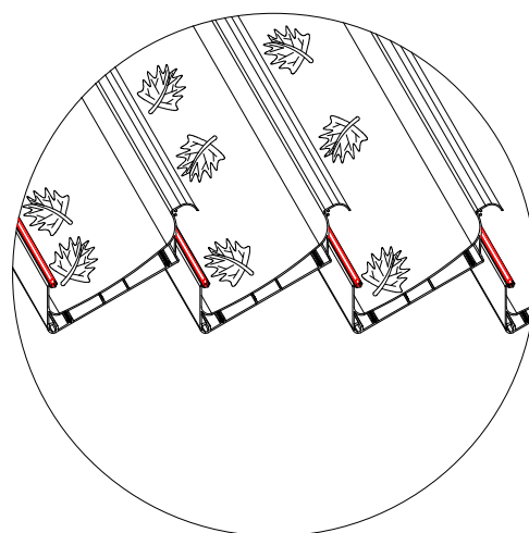
The open state of the panels, the appearance of the wicks and the special design that prevents the entry of leaves, water, etc.
