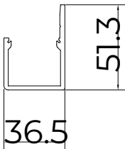
⑤ Profile for RGB Led
