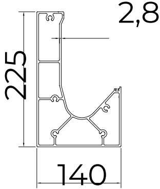
③ Front and Back Rafter & Gutter Profile
