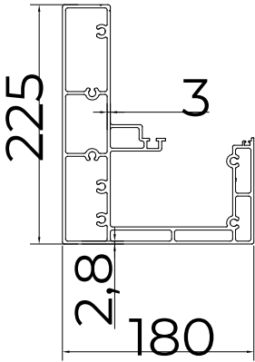
② Side Rafter & Gutter profile
