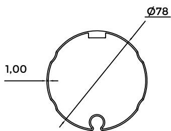
2- ROLLER TUBE \varnothing 78
