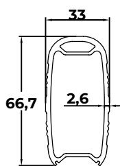
6- LIGHTING ARM PROFILE
