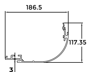
4- LOWER MAIN PROFILE
