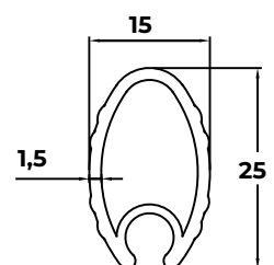
8- VALANCE WEIGHT BAR
