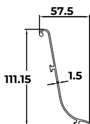
5- FABRIC PROTECTION PROFILE
