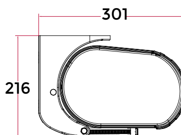
CEILING INSTALLATION BRACKET
