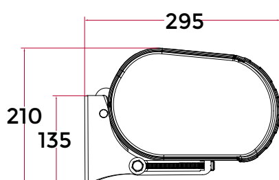
WALL INSTALLATION BRACKET
