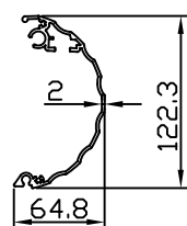
6-FRONT PROFILE
