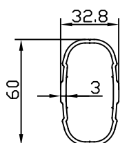
5-ARM PROFILE
