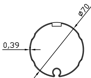
1- ROLLER TUBE Ø70
