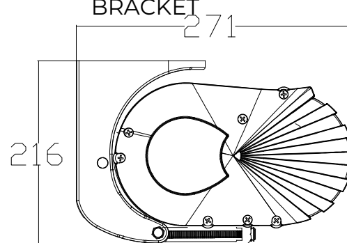
CEILING INSTALLATION BRACKET
