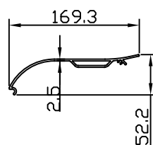
3-UPPER MAIN PROFILE
