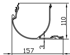
4-LOWER MAIN PROFILE
