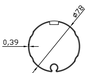
2- ROLLER TUBE Ø78
