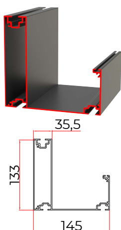
④ THICK FABRIC PROFILE
