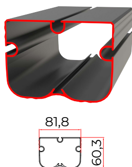
④ THICK FABRIC PROFILE
