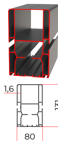
③ RAFTER PROFILE
