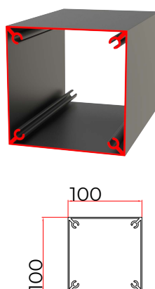
② POST PROFILE
