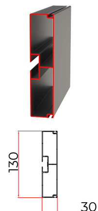
⑥ ROOF BEAM PROFILE
