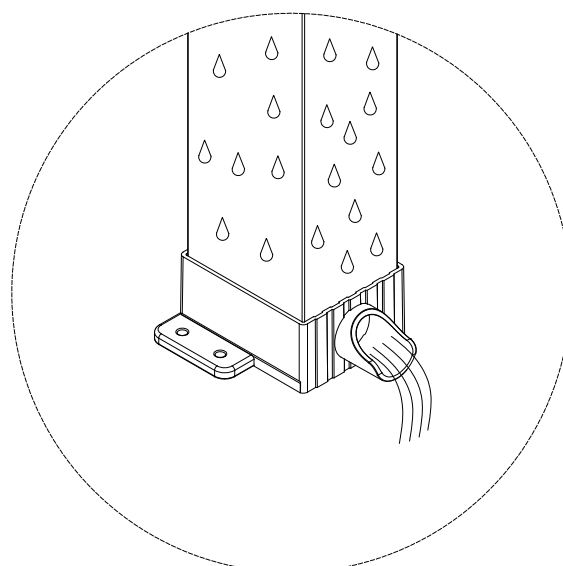
Front Post water disposal details
