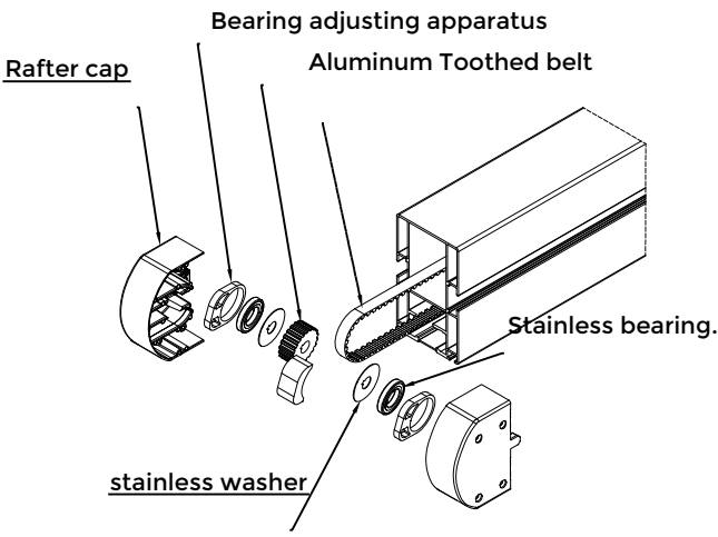
Rafter back Connector details
