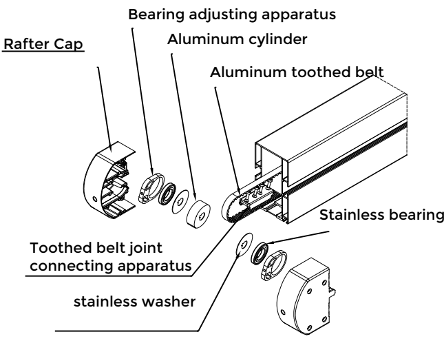
Rafter Front Connector details
