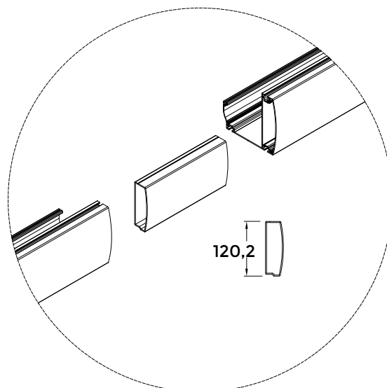
Gutter profile connecting profile detail.
