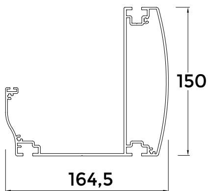
Special designed Gutter profile with increased water disposal capacity
