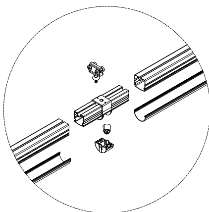
Fabric Support Profile plastic connector for middle part.
