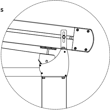
Rafter & Gutter connection detail -2
