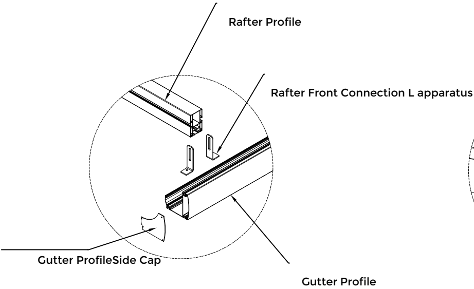
Rafter & Gutter connection detail- 1
