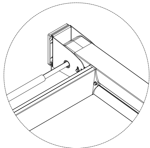
The detail of shaft profile while inserted into gear box
