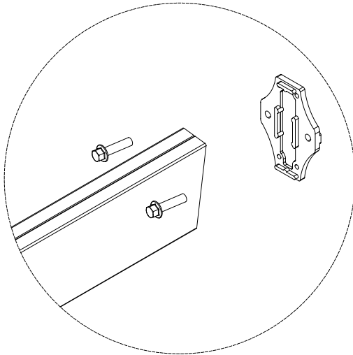
Motor and Roof Joining Profile connection details
