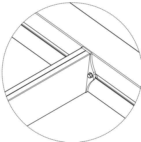
Roof Joining Profile Connection detail
