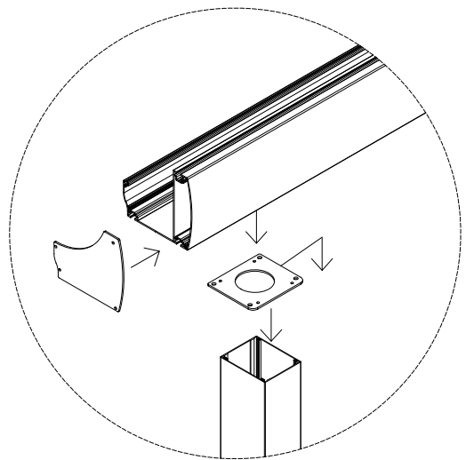
Front Post & Gutter Profile connection detail
