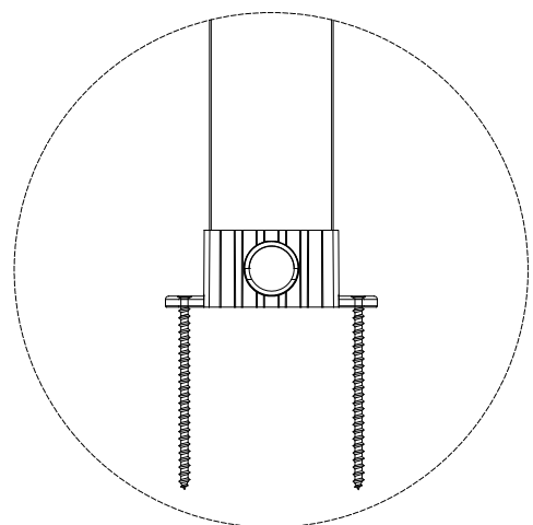
Front Post & Ground Installation Part connection detail
