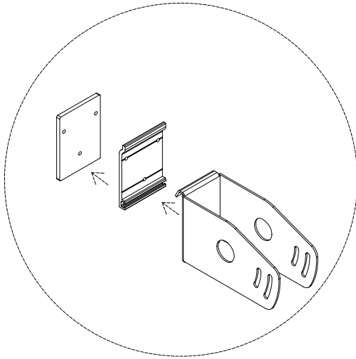
Back Rafter Connection details
