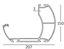
2 Gutter Profile
