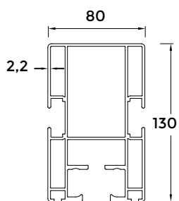
1- Rafter Profile
