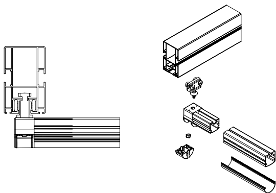
Fabric Support Profile plastic connector for sides.
