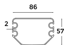
4 - Puller Profile
