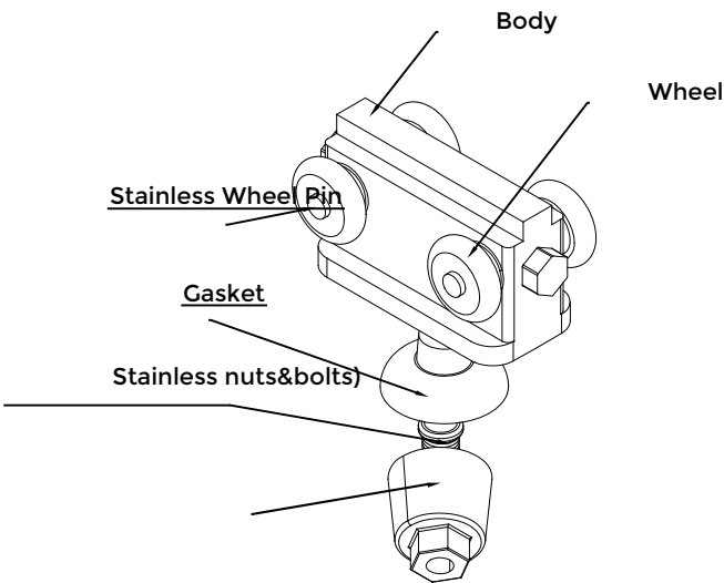
Special designed Fabric Puller Car with four wheels
