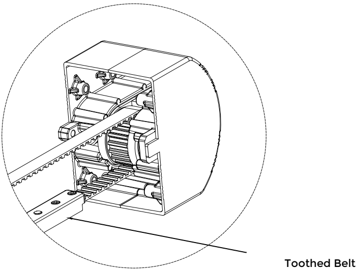
Rafter front cap interior mechanism details
