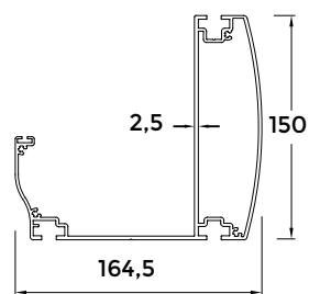
2 - Gutter Profile
