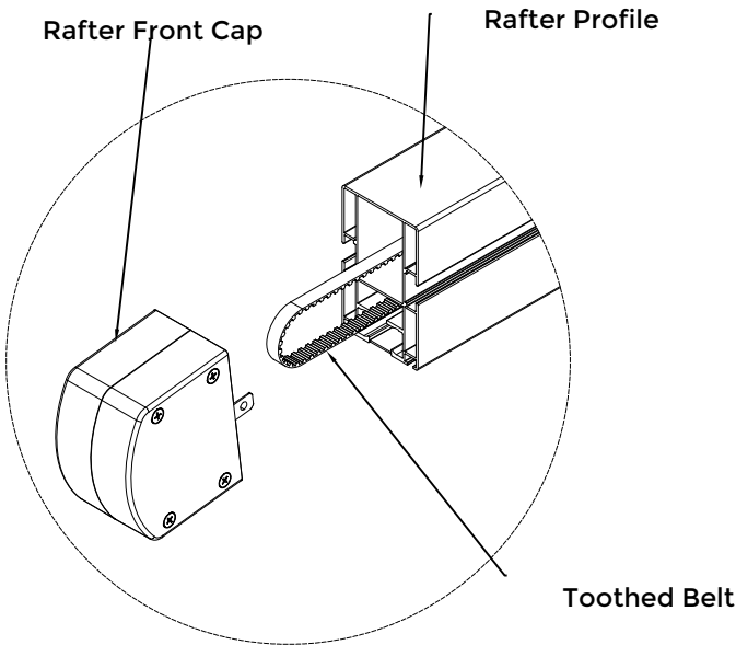
Toothed Belt operation detail
