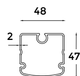
5 - Fabric Support Profile
