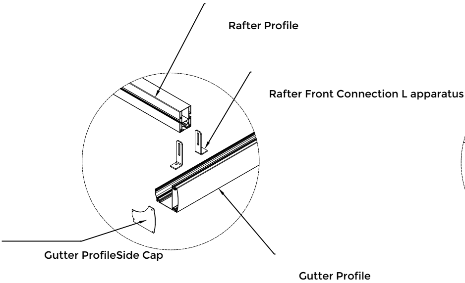
Rafter & Gutter connection detail- 1
