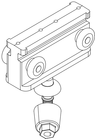
Main Puller Car
