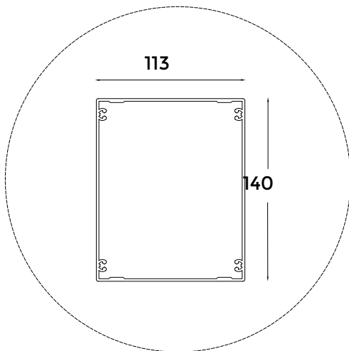
Front Post detail
