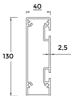
6 - Motor Profile
