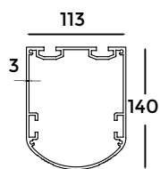
3 -Front Carrier Post
