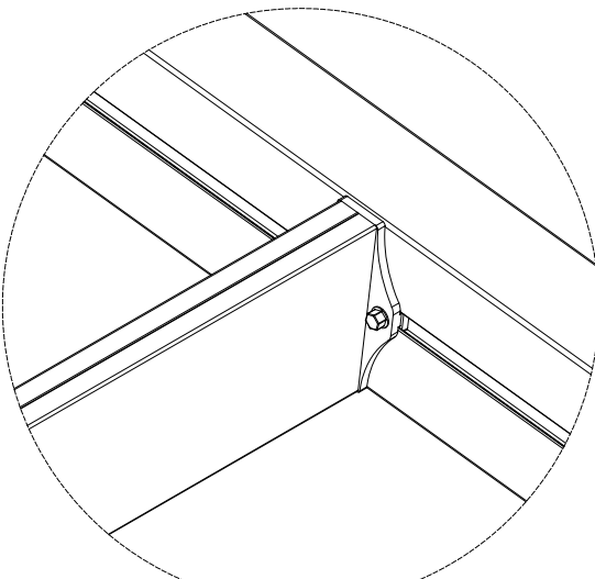
Roof Joining Profile Connection detail
