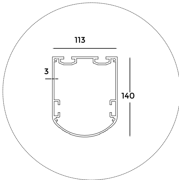
Front Post detail
