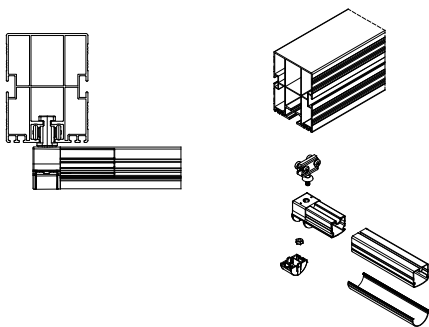
Fabric Support Profile plastic connector for sides.
