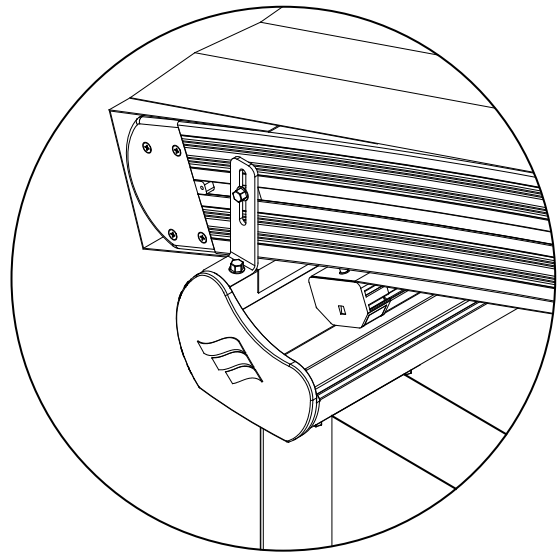
Back Rafter Detail
