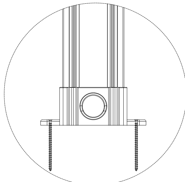
Front Post & Ground Installation Part connection detail
