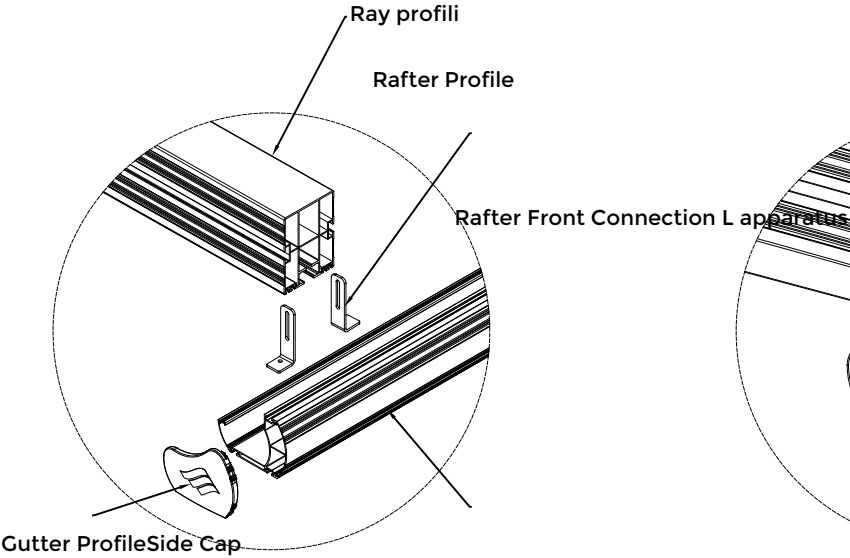
Rafter & Gutter connection detail- 1
