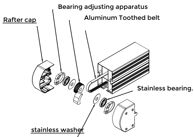
Rafter back Connector details
