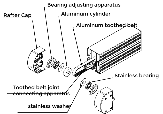
Rafter Front Connector details
