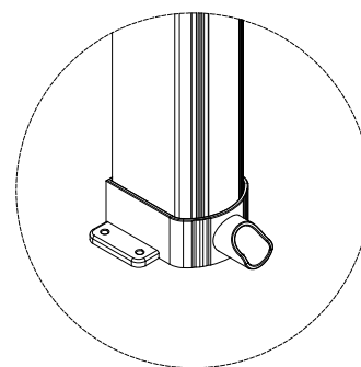
G Detailed view
