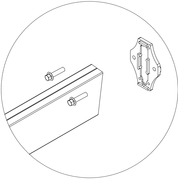
Motor and Roof Joining Profile connection details
