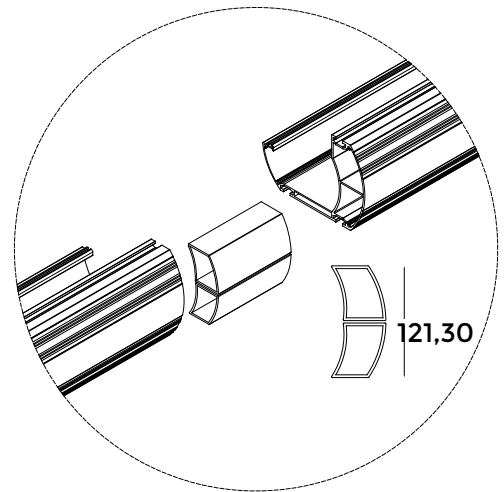
Gutter profile connecting profile detail.
