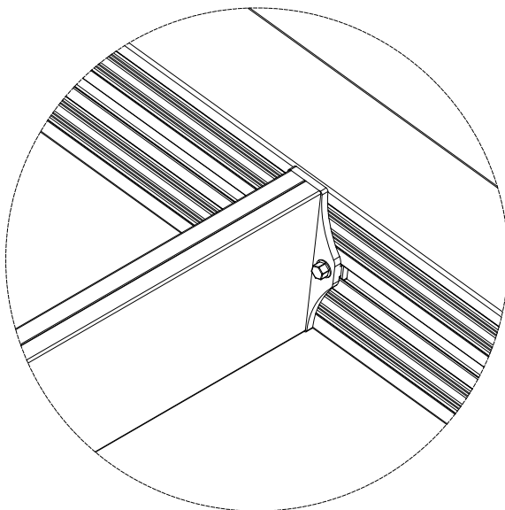
Roof Joining Profile Connection detail
