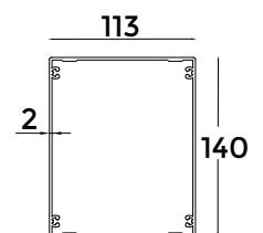
9 - Thin Shaft Profile
