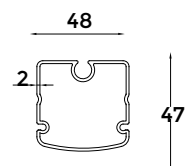
5 - Fabric Support Profile
