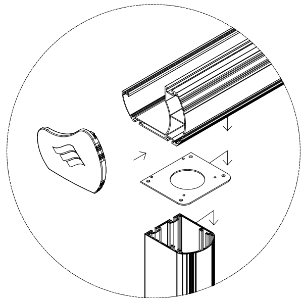
Front Post & Gutter Profile connection detail
