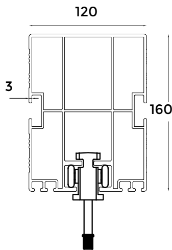
Conveyor car operating in the Rafter Profile
