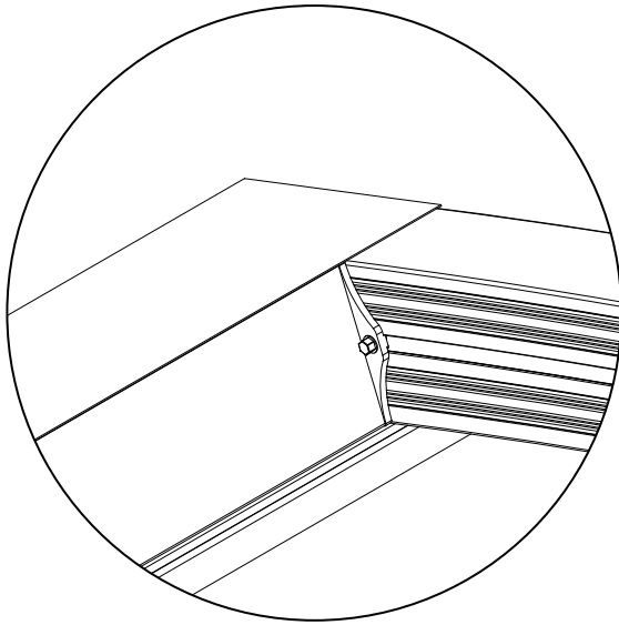
Back Rafter Connection details
