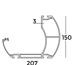
2 - Gutter Profile
