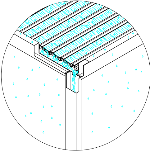
Drainage of water from louvres with the help of gutter to the post
