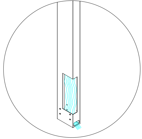
Evacuation of water in the posts
