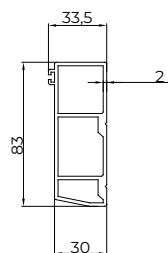
4 Front profile
