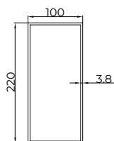
2 Carrier post and Rafter profile
