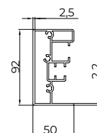
3 Rafter profile
