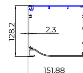
6 Motor box
