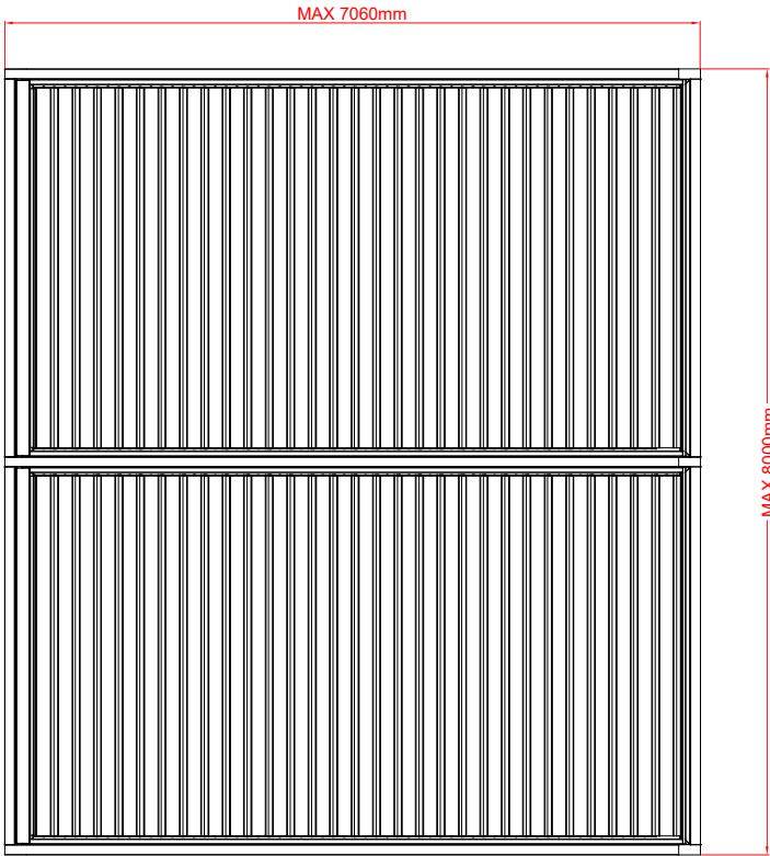
Double module system measurements
