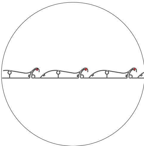
The wicks that provide sealing when louvres are closed
