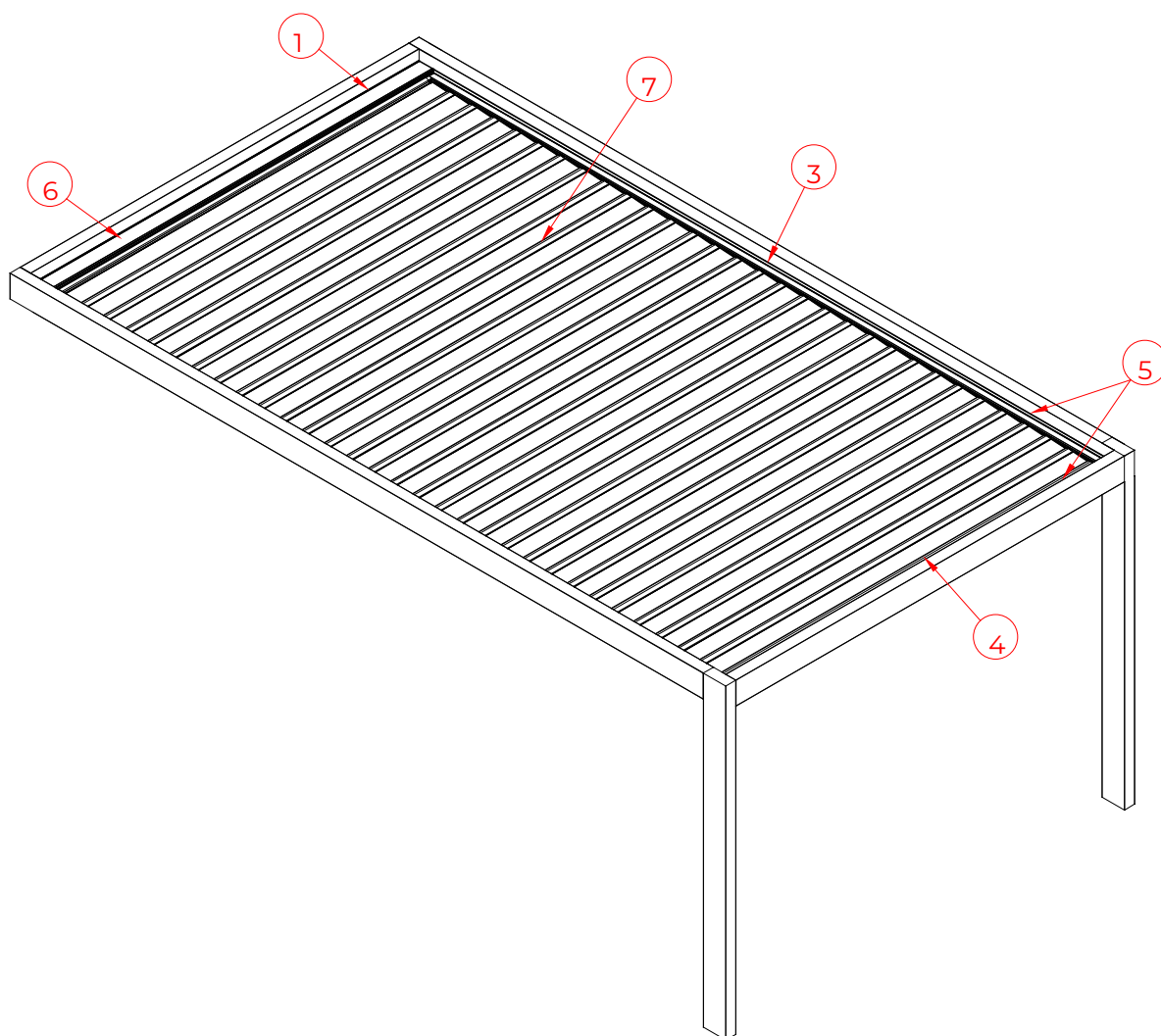
1 Back gutter profile
