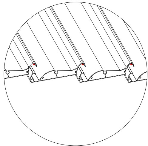
Wicks when louvres are open
