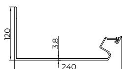
1 Back gutter profile
