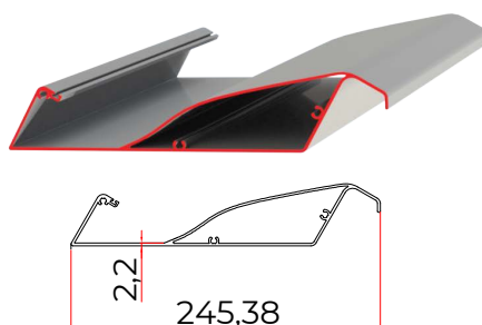
⑦ LOUVRE PROFILE
