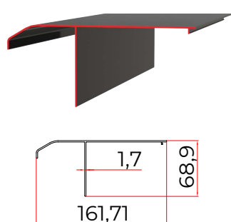
⑦ LOUVRE PROFILE
