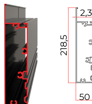
③ SIDE PROFILE
