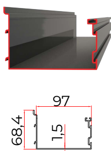
④ GUTTER PROFILE
