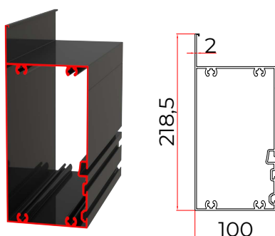
① FRONT/BACK PROFILE
