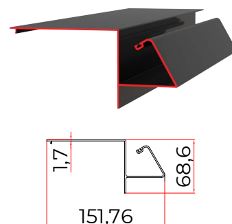
⑥ FRONT CLOSING PROFILE
