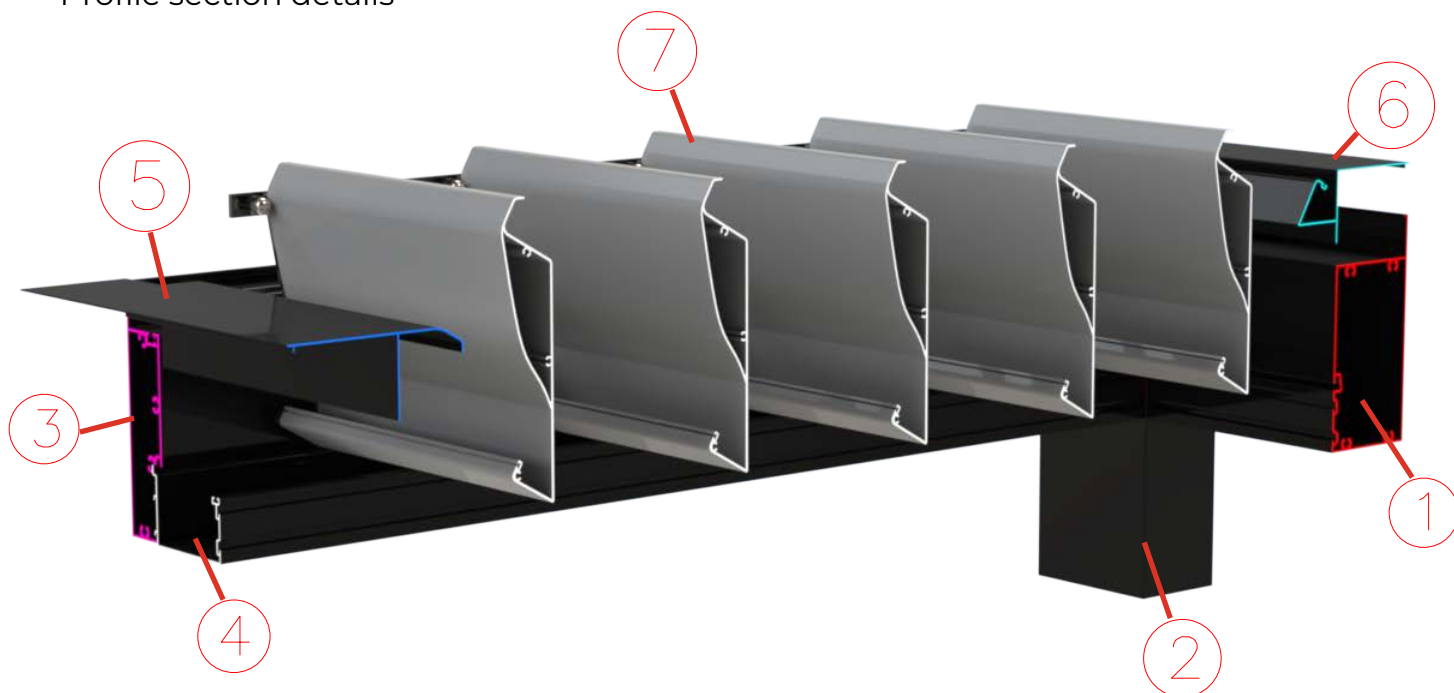
① FRONT/BACK PROFILE
