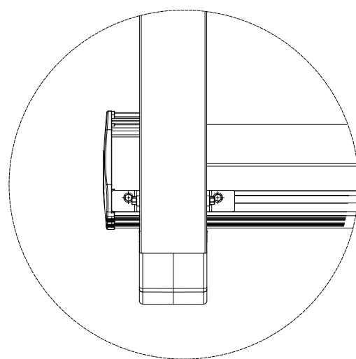
Rafter & Gutter connection detail- 4
