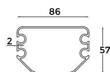
4 - Puller Profile
