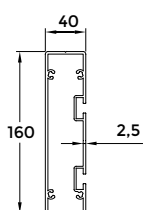
6 - Motor Profile
