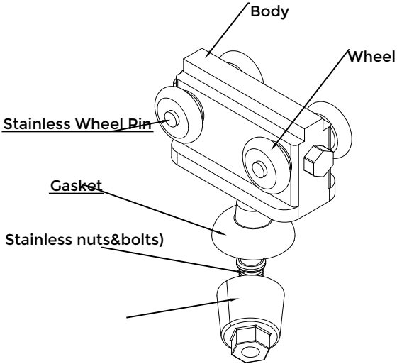
Special designed Fabric Puller Car with four wheels
