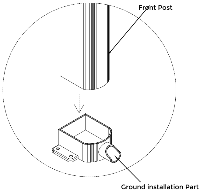
Ground Installation Part detail
