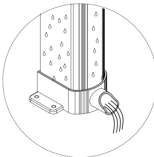
Front Post water disposal details
