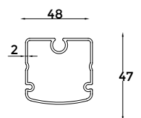
5 - Fabric Support Profile
