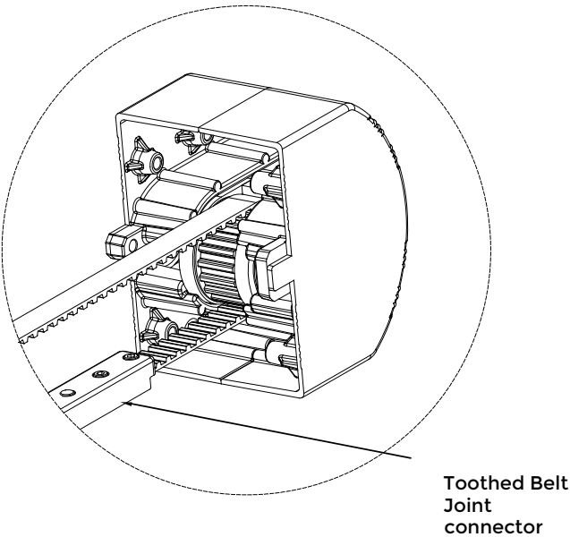
Rafter front cap interior mechanism details
