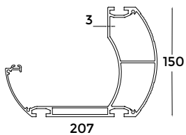
2 - Gutter Profile
