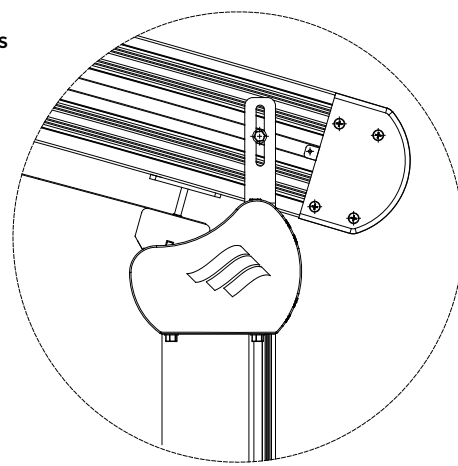
Rafter & Gutter connection detail -2
