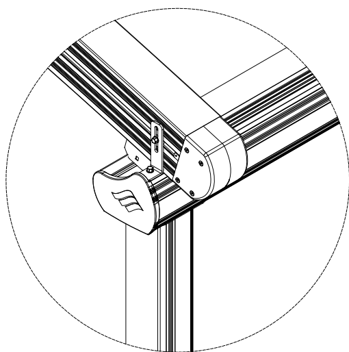
Rafter & Gutter connection detail- 3
