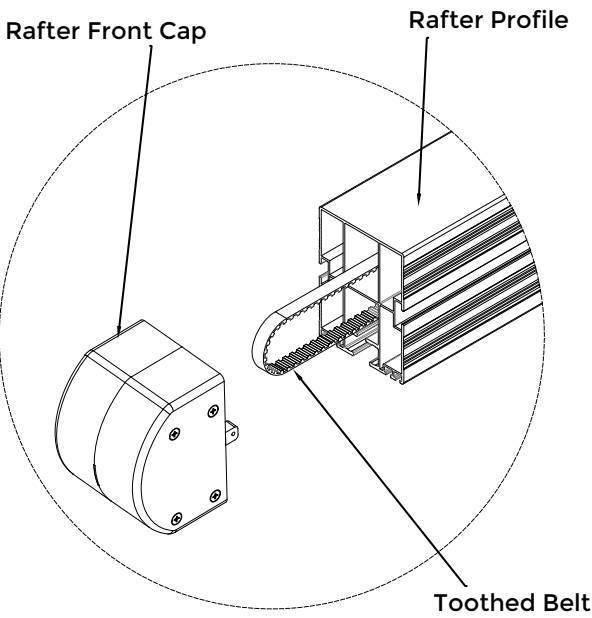
Toothed Belt operation detail
