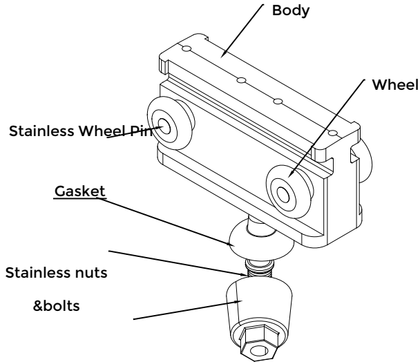
Special designed Main Puller Car with four wheels
