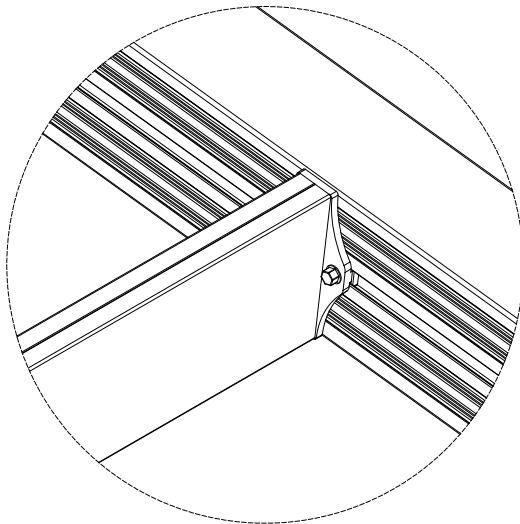
Roof Joining Profile Connection detail
