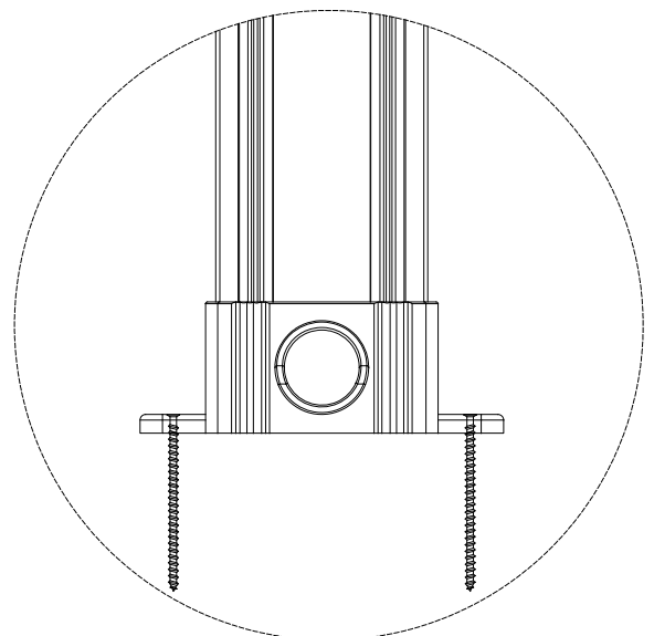
Front Post & Ground Installation Part connection detail
