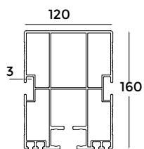
1- Rafter Profile
