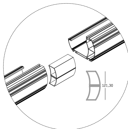
Gutter profile connecting profile detail.
