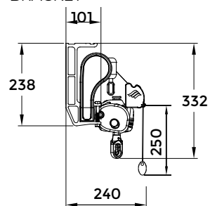
CEILING INSTAALATION BRACKET
