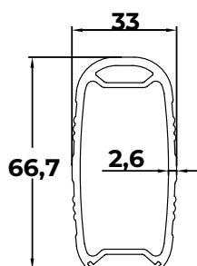
4- LIGHTING ARM PROFILE
