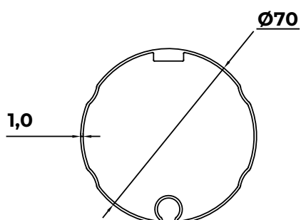
1- ROLLER TUBE \varnothing 70
