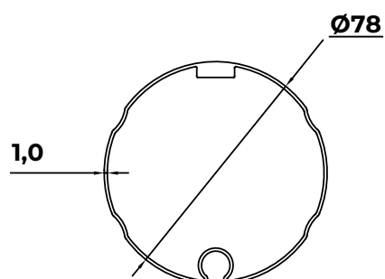
2- ROLLER TUBE \varnothing 78
