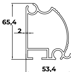
5- FRONT PROFILE
