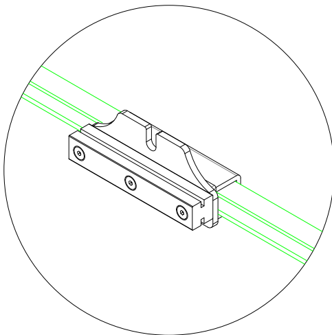
Front lock mechanism and timing belt assembly tool set.
