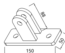
⑥ Rail hanger bracket
