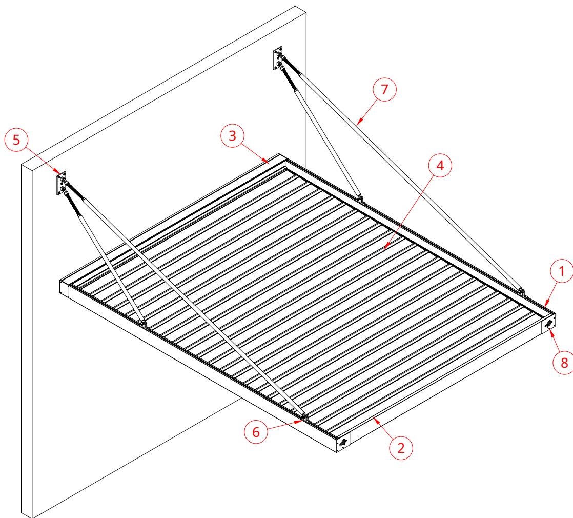
① Grooved rail profile
