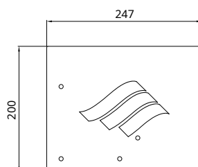
⑧ Front cover
