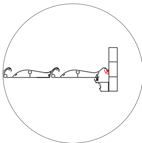
Front side detail
