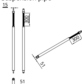
⑦ Suspension pipe
