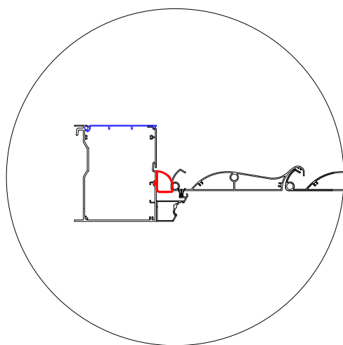
Back side detail
