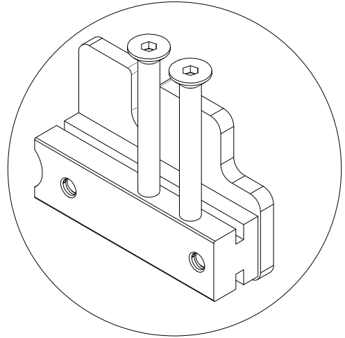
Rear locking mechanism
