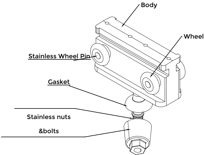
Special designed Main Puller Car with four wheels
