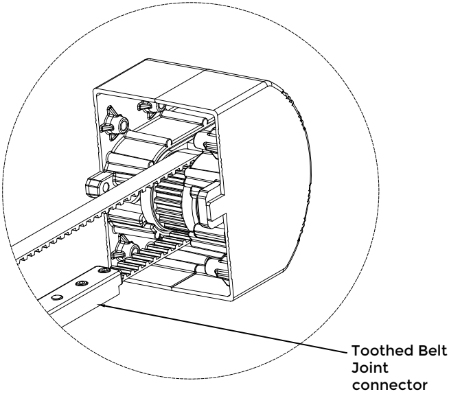
Rafter front cap interior mechanism details
