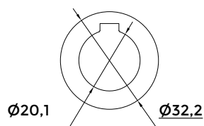
8 -Thick Shaft Profile
