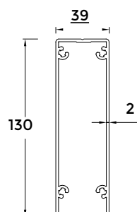
7 - Roof Joining Profile
