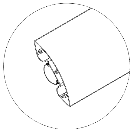
B-Sun Blocker detailed view- with channel for lighting system
