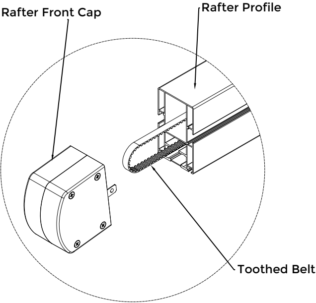
Toothed Belt operation detail
