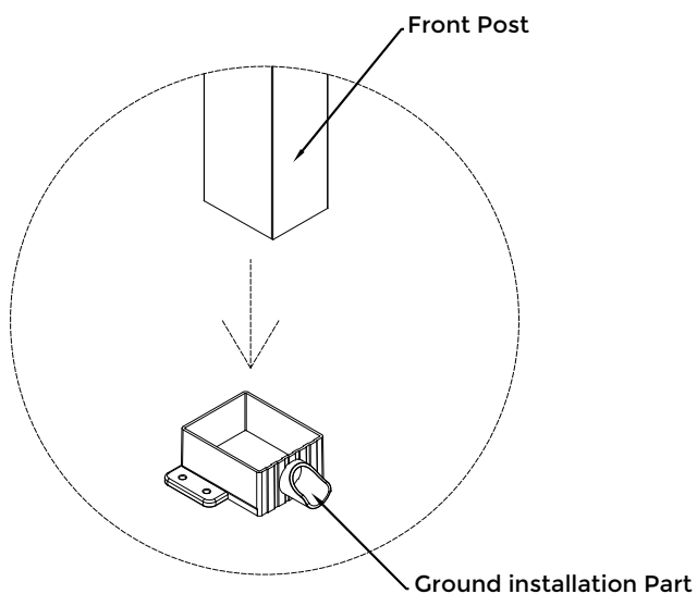
Ground Installation Part detail
