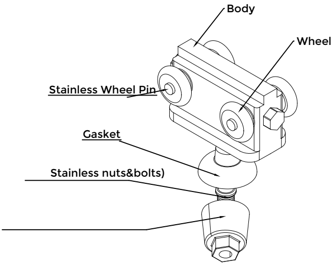
Special designed Fabric Puller Car with four wheels
