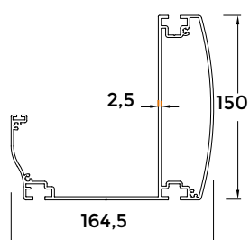
2 - Gutter Profile
