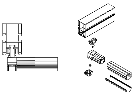
Fabric Support Profile plastic connector for sides.
