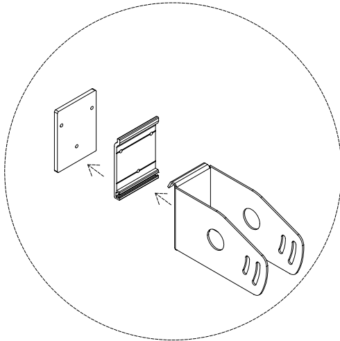
Back Rafter Connection details
