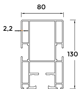
1- Rafter Profile
