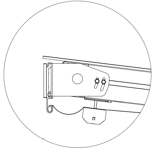
Back Rafter Detail
