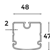
5 - Fabric Support Profile
