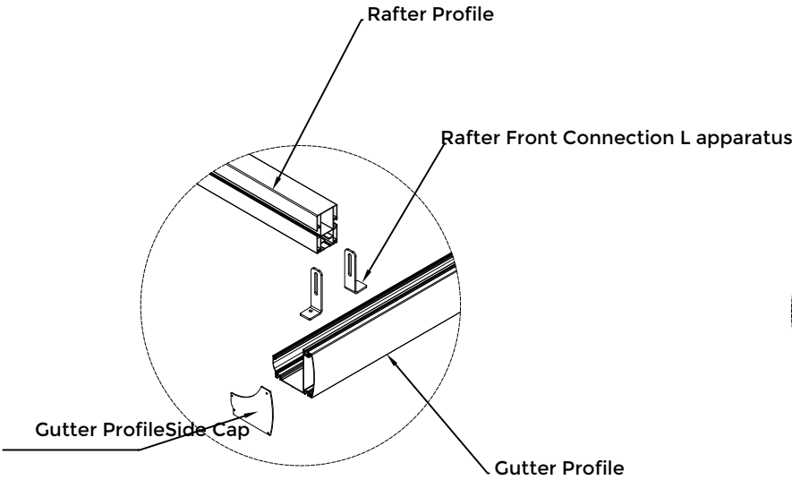
Rafter & Gutter connection detail- 1
