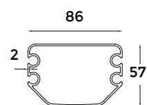
4 - Puller Profile
