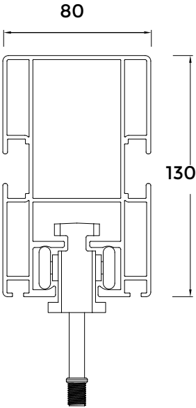
Conveyor car operating in the Rafter Profile
