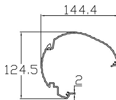
3- MAIN PROFILE
