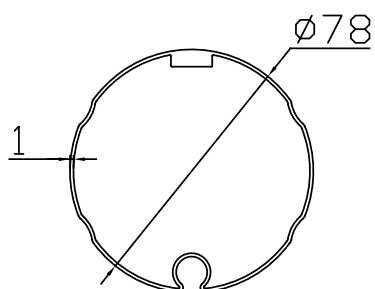
2- ROLLER TUBE Ø78
