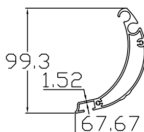
5- FRONT PROFILE
