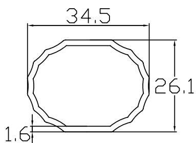
4- ARM PROFILE
