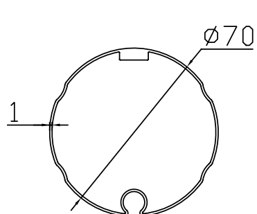
1- ROLLER TUBE Ø70
