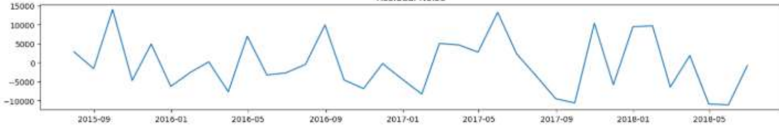
Residual Noise
