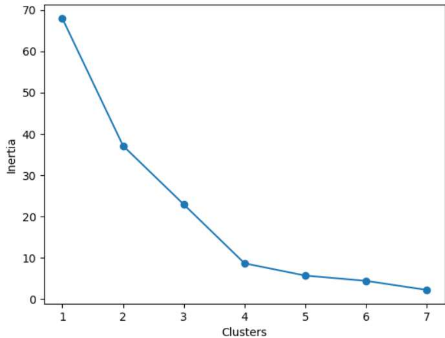
Elbow Method
