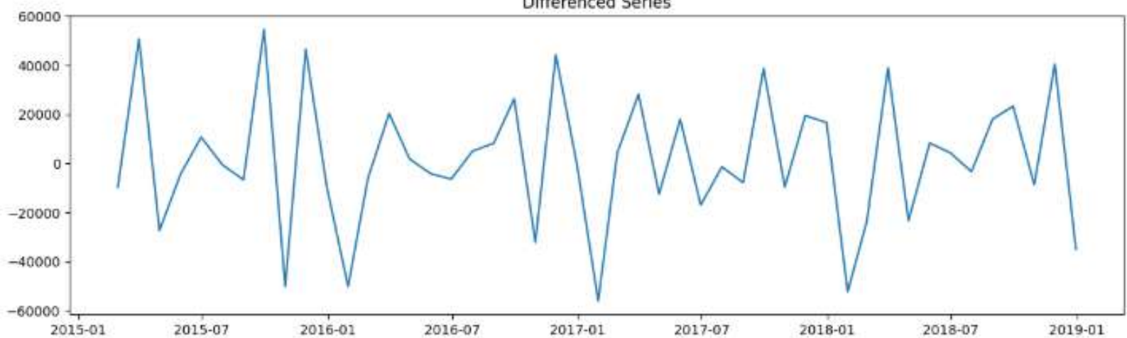
Differenced Series
