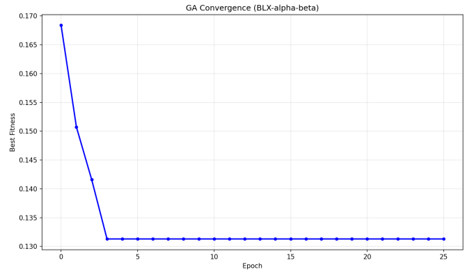
Fig. 4. GA convergence over 25 epochs. The fitness stabilized by epoch 3.
