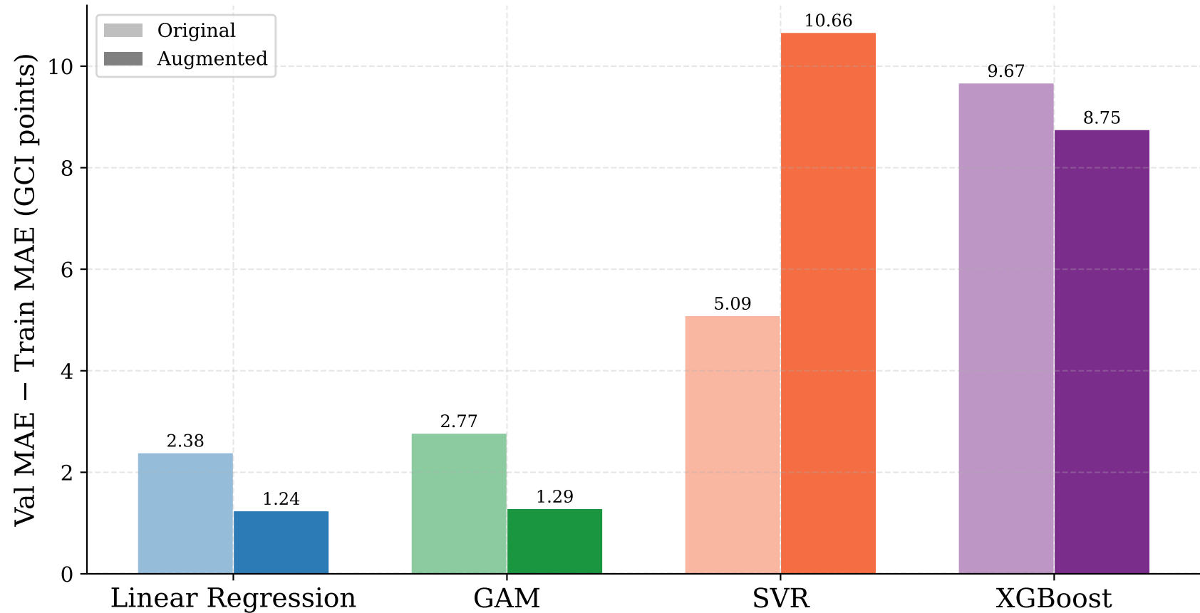
Train-Validation MAE Gap: Original vs Augmented
