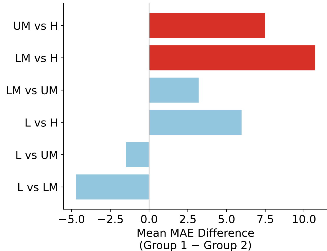
XGBoost
