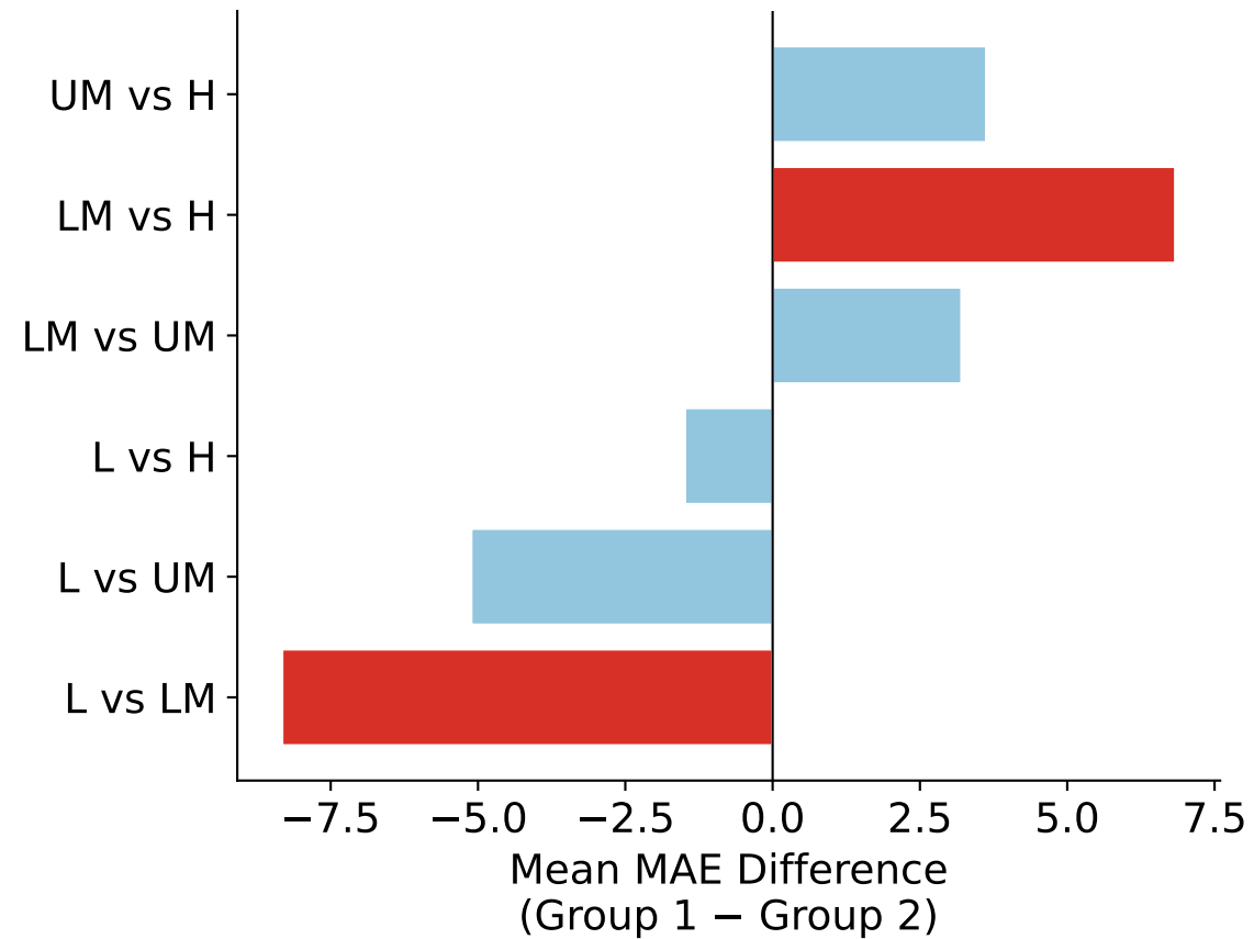
XGBoost
