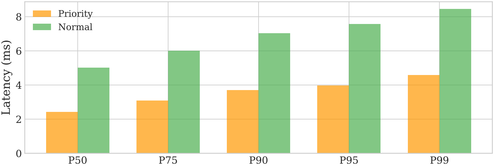
Latency Percentiles Comparison
