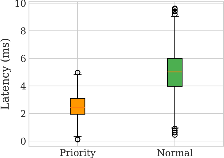
Latency by Traffic Type
