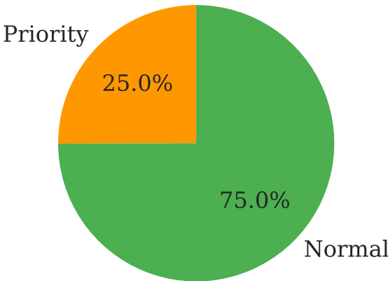
Packet Distribution
