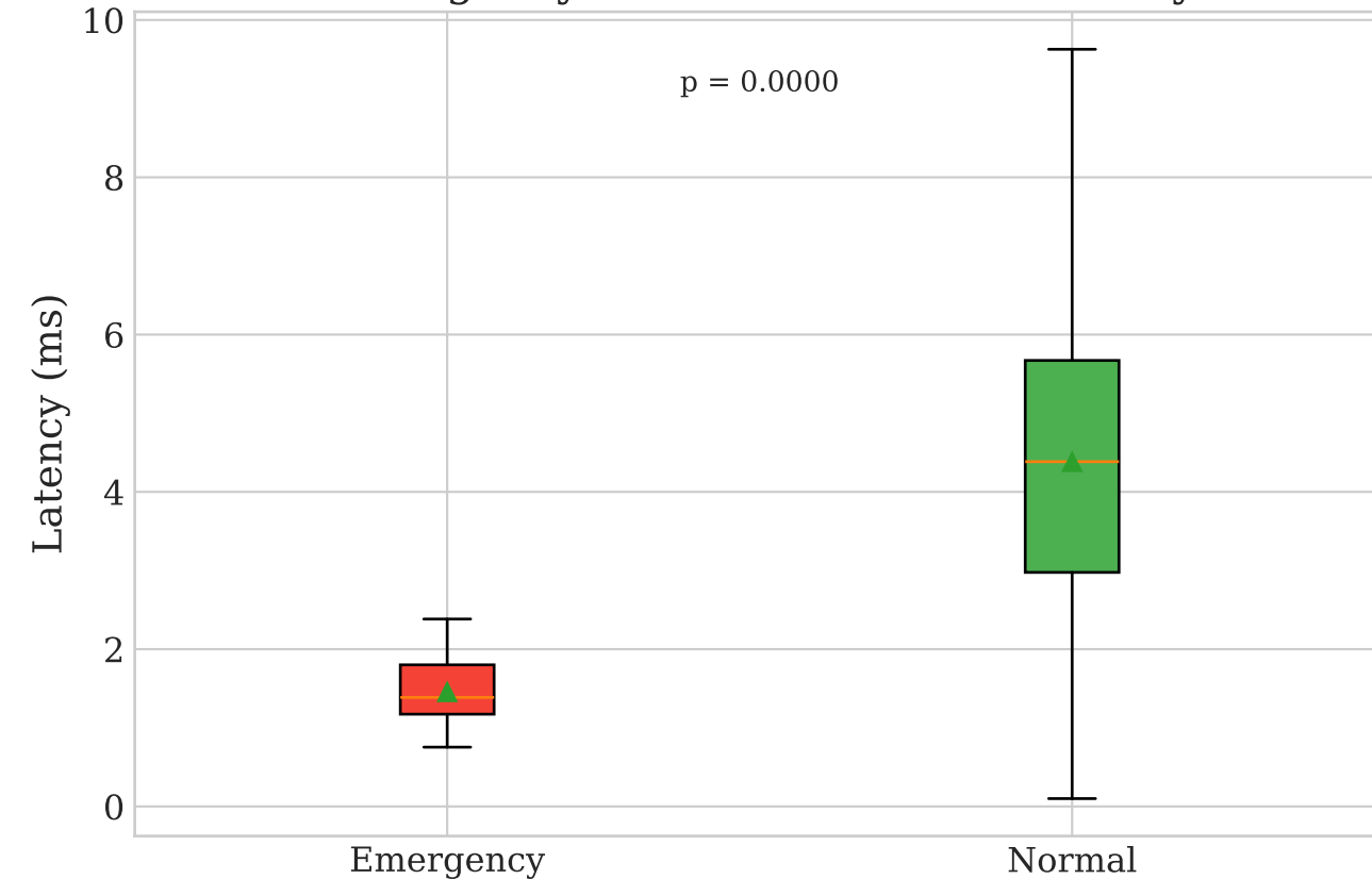
Emergency vs Normal Traffic Latency
