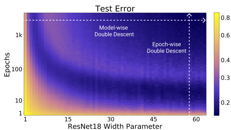
Fig. 2 (left), test error. Test error attains \approx 0.47 at width k \approx 10 and decreases to \approx 0.24 at k = 64 .
