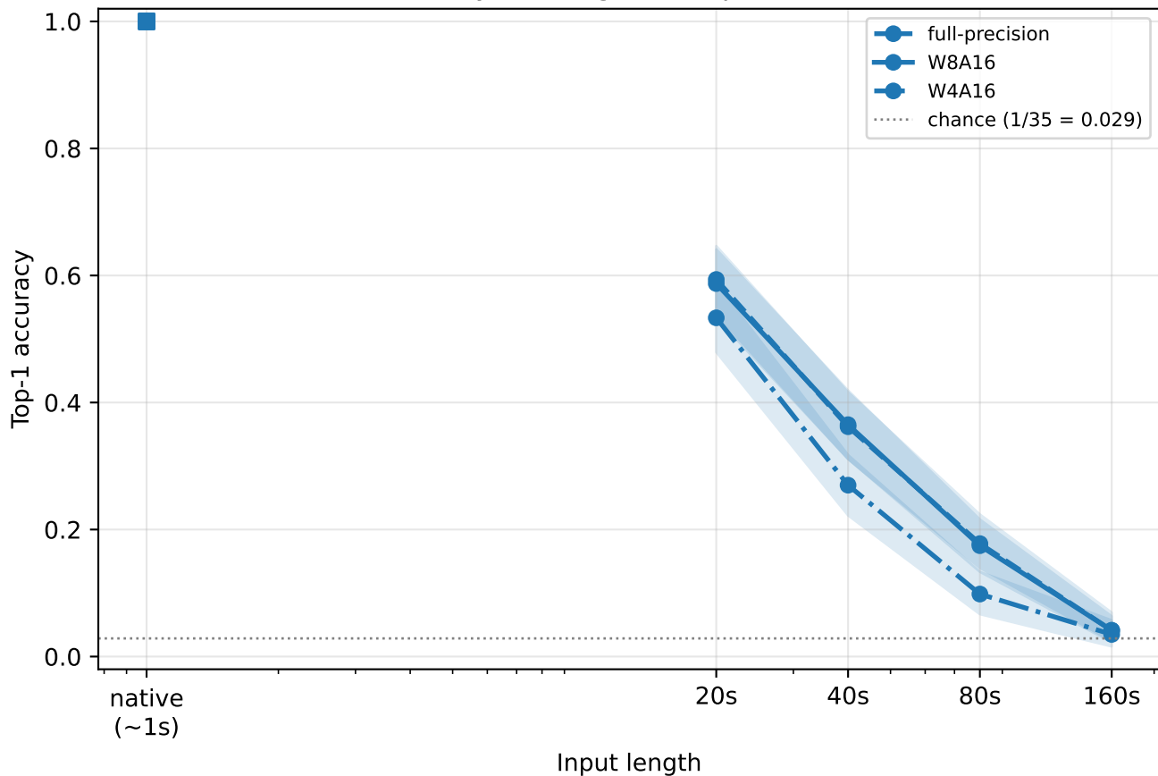
AST: accuracy vs. length (3 clips/class, 95% CI)
