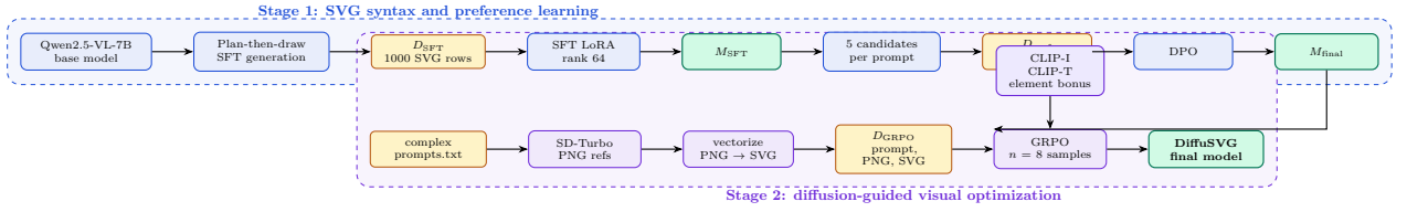
Figure 1: End-to-end DiffuSVG pipeline. Stage 1 learns SVG syntax and preference structure. Stage 2 uses diffusion-generated reference images and a CLIP-based reward to improve complex scene fidelity.
