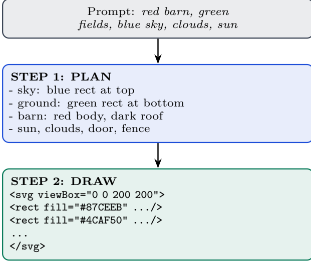
Figure 2: Plan-then-draw prompting. Planning acts as a scratchpad that commits the model to multiple objects before it starts producing SVG tokens.
