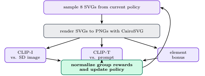
Figure 4: GRPO reward loop. SVG candidates are rendered before scoring, making the reward visual rather than purely syntactic.
