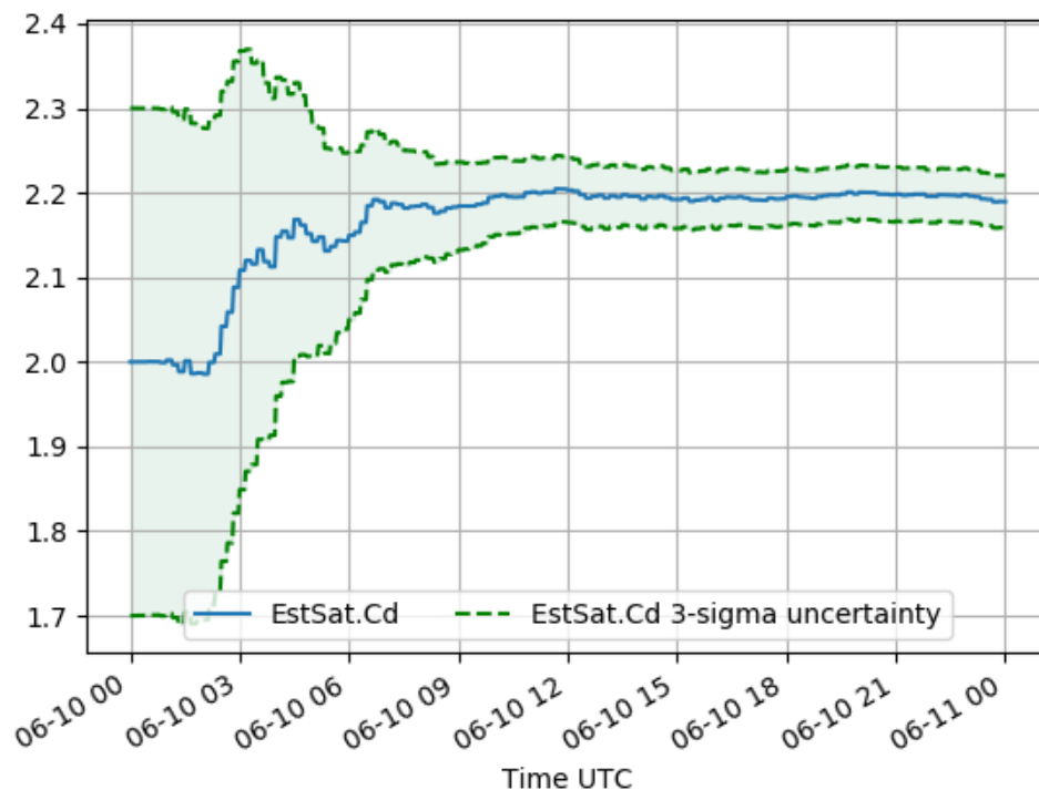
Filter EstSat.Cd and 3-Sigma Uncertainty
