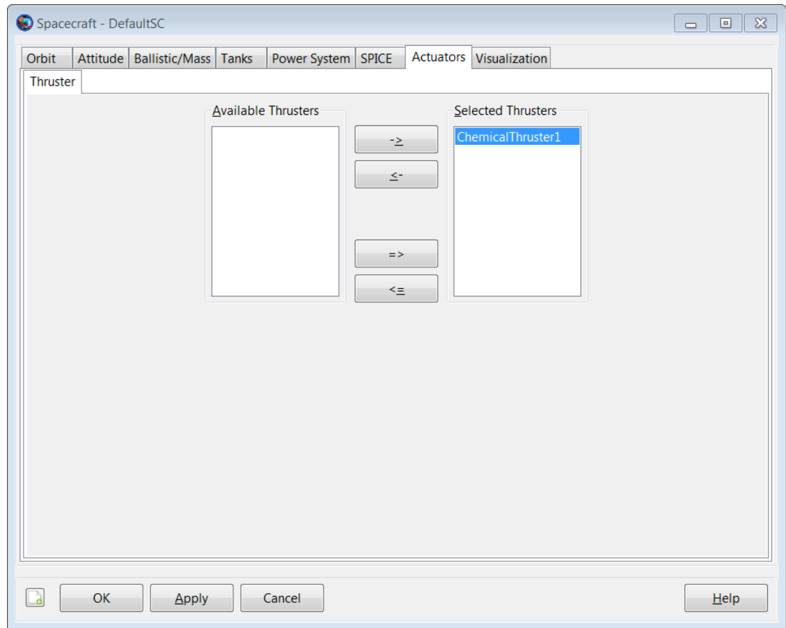
Figure 33. Attach ChemicalThruster1 to DefaultSC
