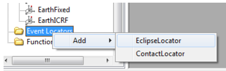
Figure 104. Location of EclipseLocator
