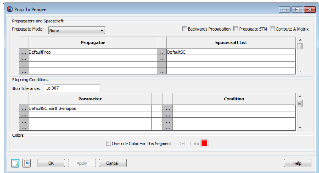
Figure 36. Prop To Perigee Command Configuration
