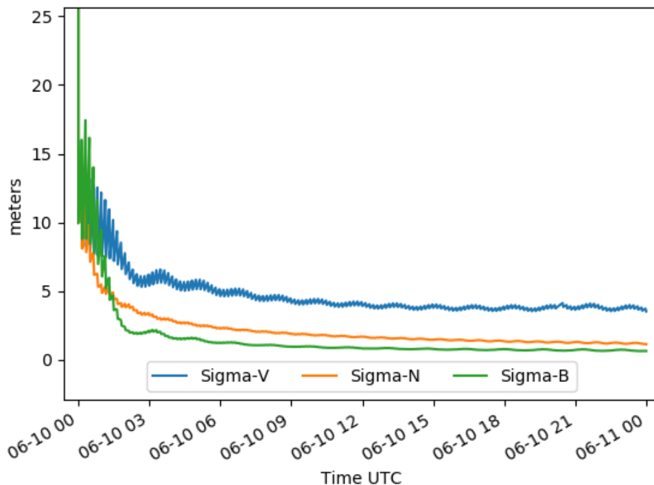
Filter 1-Sigma Position Uncertainty
