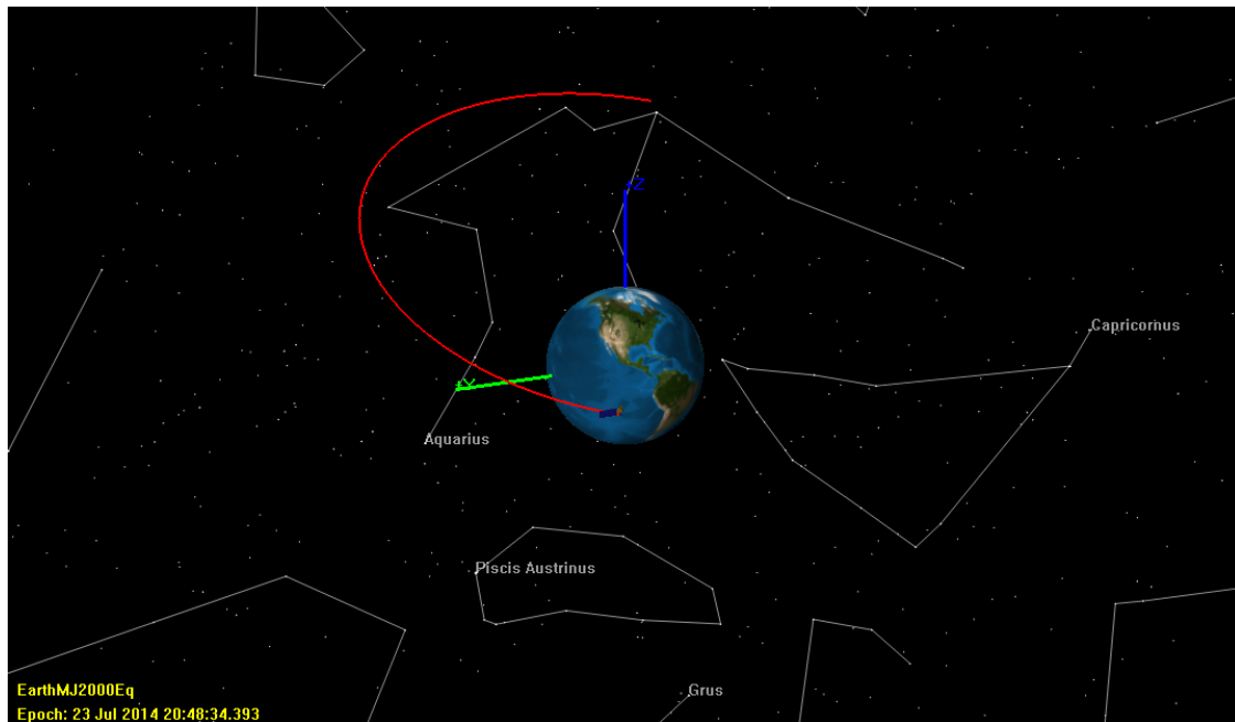
Figure 17. Orbit View Plot after Mission Run
