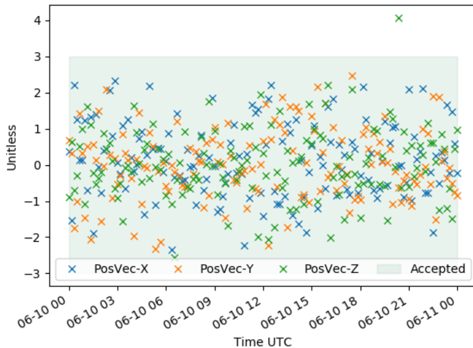
Filter Scaled Residuals
