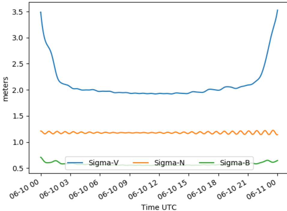
Smoother 1-Sigma Position Uncertainty
