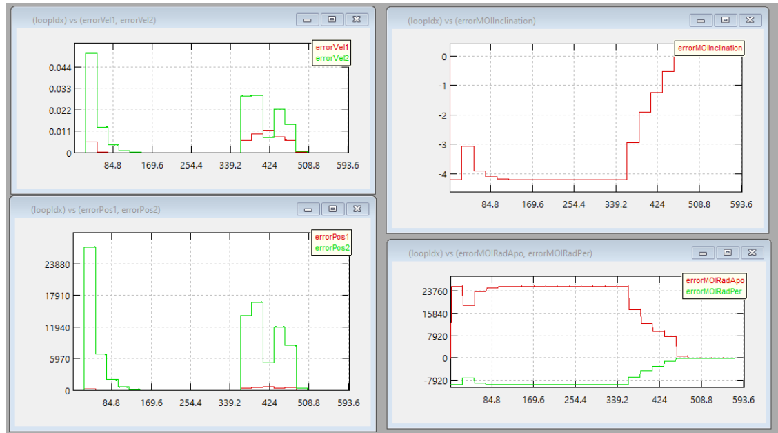
Figure 82. Solution Using New Guess
