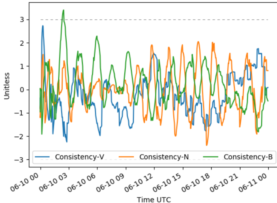
Filter-Smoother Position Consistency
