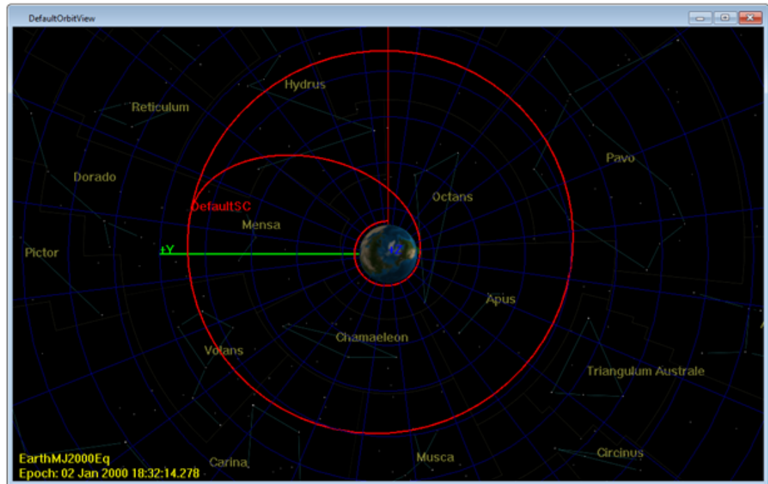
Figure 28. 3D View of Hohmann Transfer
