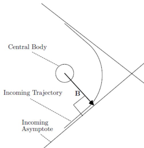
Figure 84. The B-vector as seen from a viewpoint perpendicular to orbit plane
