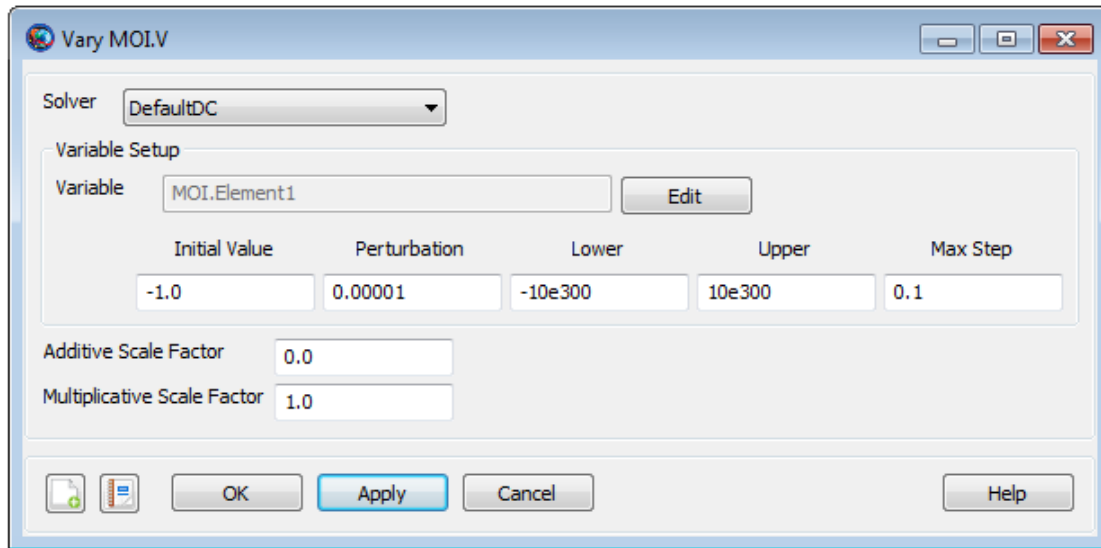
Figure 96. Vary MOI Command Configuration
