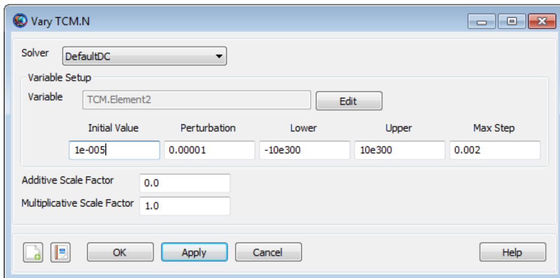
Figure 54. Vary TCM.N Command Configuration
