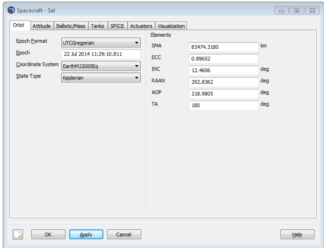
Figure 12. Spacecraft State Setup
