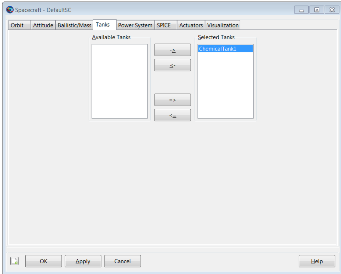
Figure 32. Attach ChemicalTank1 to DefaultSC
