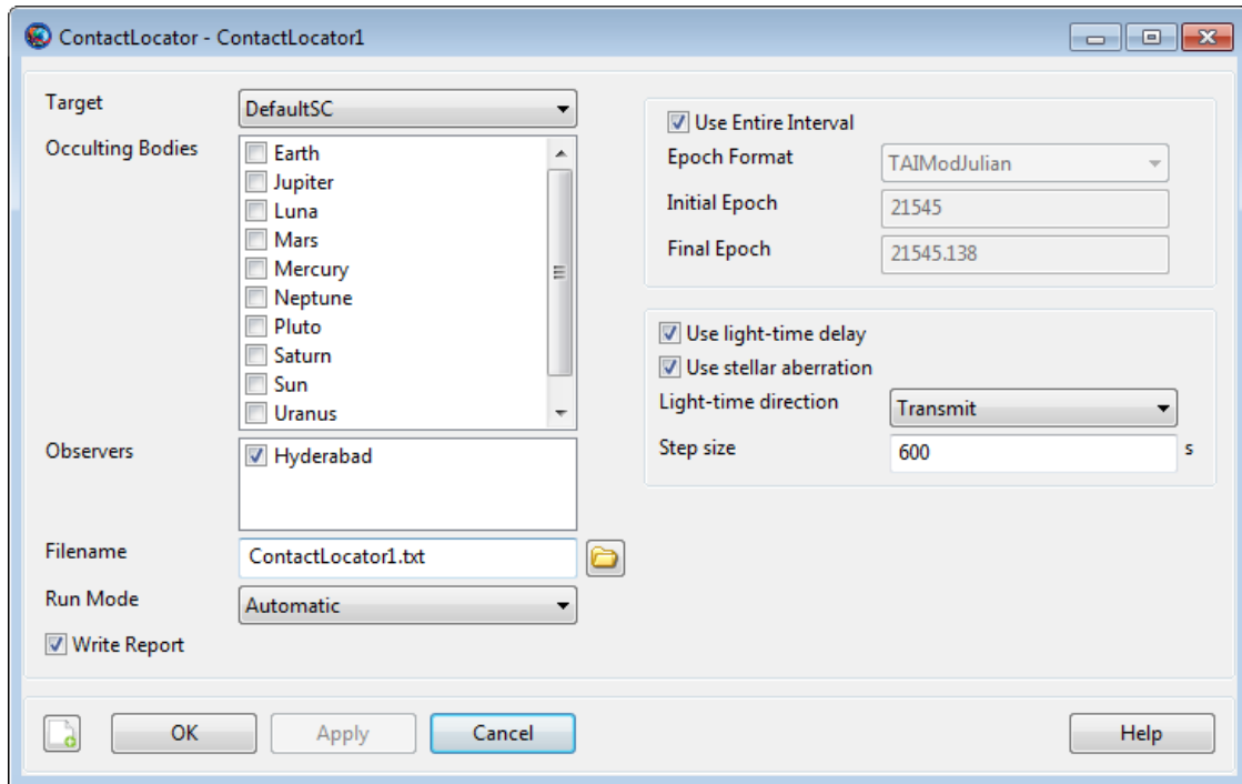
Figure 109. ContactLocator Configuration Window
