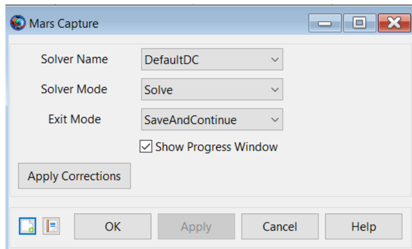
Figure 67. Mars Capture Command Configuration
