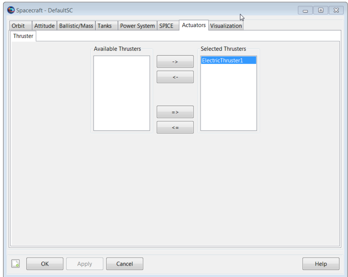
Figure 115. Attach ElectricThruster1 to DefaultSC
