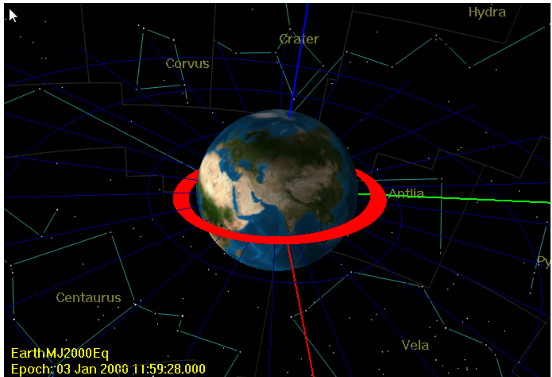
Figure 120. 3D View of Finite Electric Maneuver
