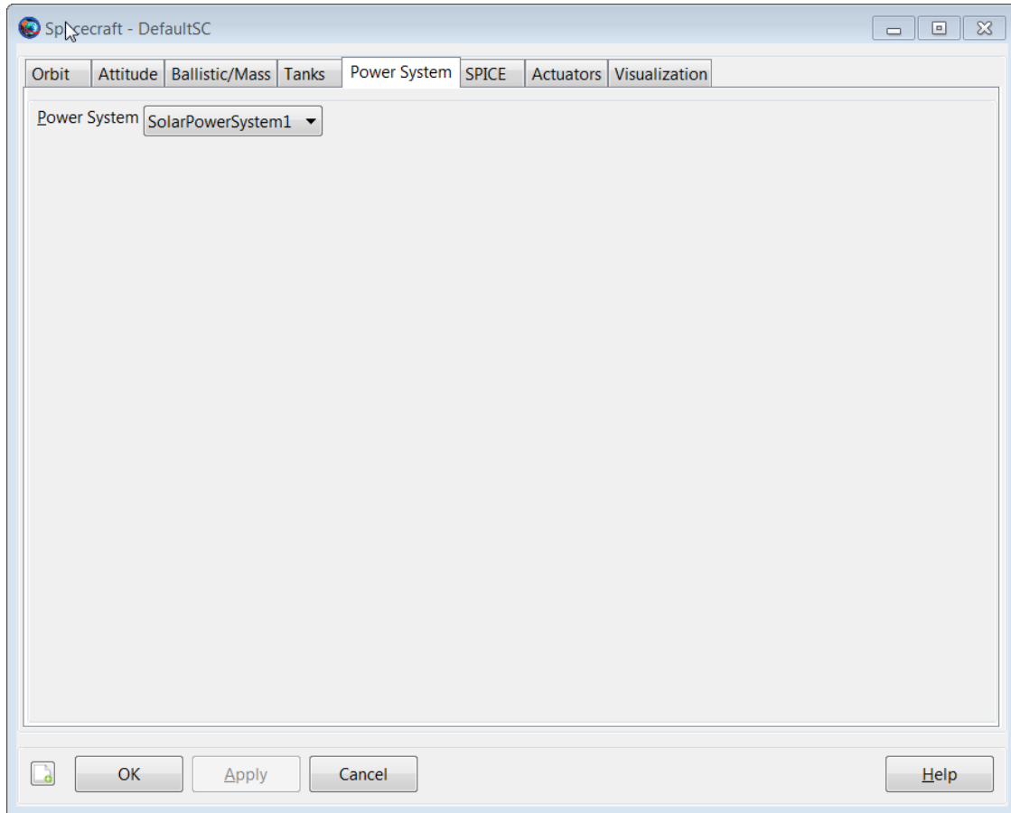
Figure 116. Attach SolarPowerSystem1 to DefaultSC
