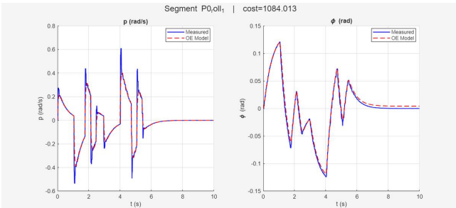
System Identification Diagnostic Plot
