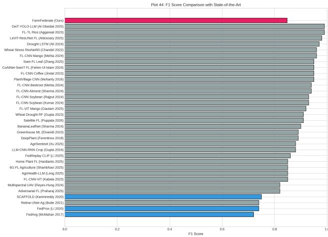
Fig. 23: Comparison with state-of-the-art approaches in agricultural stress detection. FarmFederate’s VLM fusion ( F1 = 0.848 ) achieves competitive performance while uniquely offering privacy-preserving federated training and multimodal fusion.
