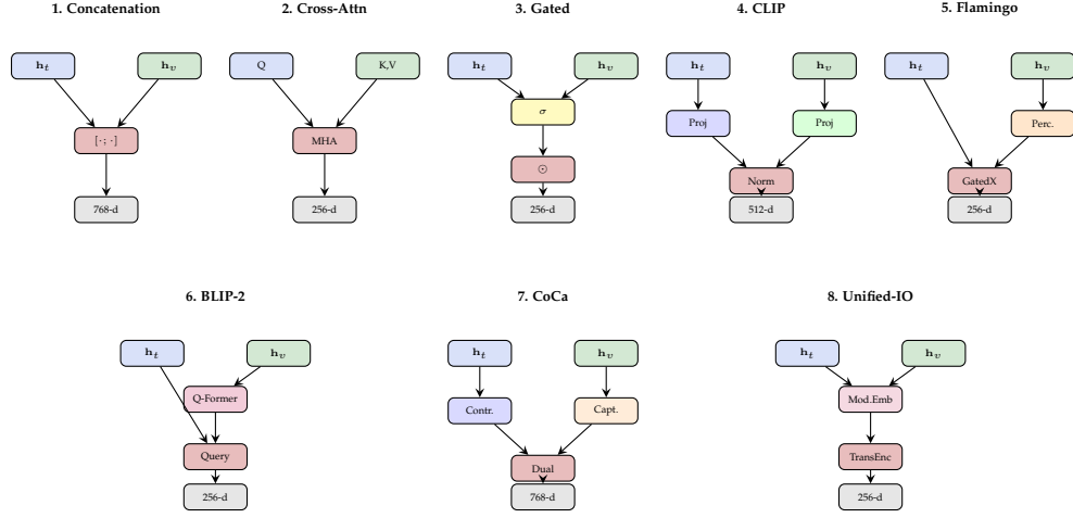
Fig. 3: Eight VLM fusion architectures: (1) Concatenation, (2) Cross-Attention, (3) Gated Fusion, (4) CLIP-style contrastive alignment, (5) Flamingo perceiver with gated cross-attention, (6) BLIP-2 Q-Former, (7) CoCa dual contrastive-captioning, and (8) Unified-IO modality embeddings with transformer encoder.
