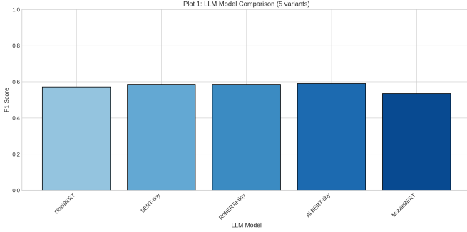
Fig. 6: F1 score comparison across five LLM text encoder variants. ALBERT-tiny achieves the highest score (0.590), while all models remain within a narrow performance band (0.53–0.59), indicating comparable text encoding capacity.
