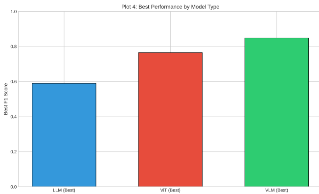
Fig. 18: Cross-paradigm F1 comparison for Federated LLM, Federated ViT, and Federated VLM (centralized and federated). Federated VLM (green) achieves the highest absolute F1 (0.848 centralized, 0.785 federated); Federated LLM (blue) incurs the smallest accuracy penalty under federation (92.9% retention); Federated ViT (red) delivers strong unimodal performance (0.765) but is most affected by non-IID partitioning (86.1% retention).
