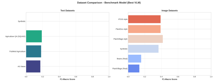
Fig. 5: Combined dataset comparison showing model performance across different text sources (AG News, PubMed, SQuAD) and image datasets (PlantVillage, Beans, synthetic variants). Cross-modal combinations reveal complementary strengths between modalities.
