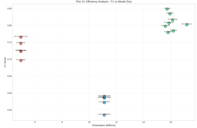
Fig. 19: F1 score vs. model size (number of parameters) across all architectures. ViT models (~5M params) achieve strong F1 (0.70–0.77), LLM models (~11M) achieve moderate F1 (0.53–0.59), while VLM models (16–17M) reach the highest F1 (0.78–0.85), demonstrating that multimodal fusion justifies the additional parameter cost.
