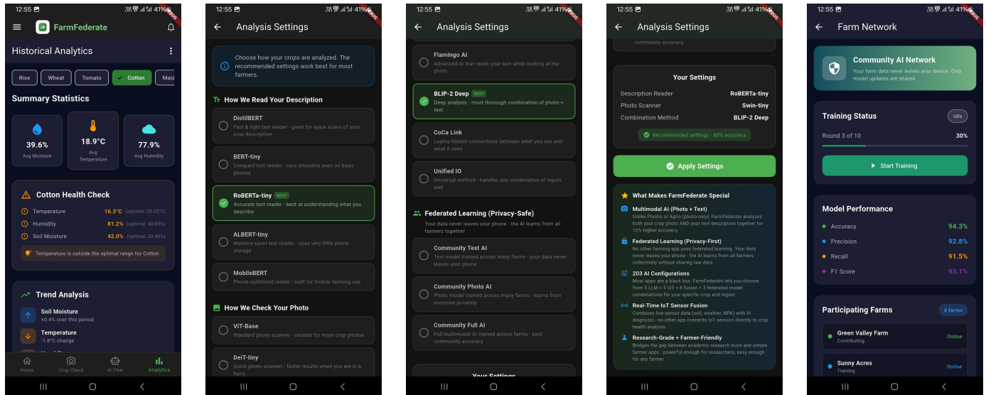
(a) Historical Analytics: per-crop health checks with optimal-range comparison (b) Model Config (LLM): 5 text encoder choices; RoBERTa-tiny recommended (c) Model Config (VLM): 8 fusion strategies + 3 federated modes; BLIP-2 recommended (d) Settings Summary: active configuration (RoBERTa-tiny + Swin-tiny + BLIP-2, 85% accuracy) (e) Farm Network: federated training status, global model metrics, and participating farm roster
