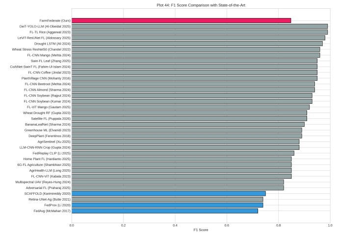
Fig. 23: Comparison with state-of-the-art approaches in agricultural stress detection. FarmFederate’s VLM fusion (F1=0.848) achieves competitive performance while uniquely offering privacy-preserving federated training and multimodal fusion.
