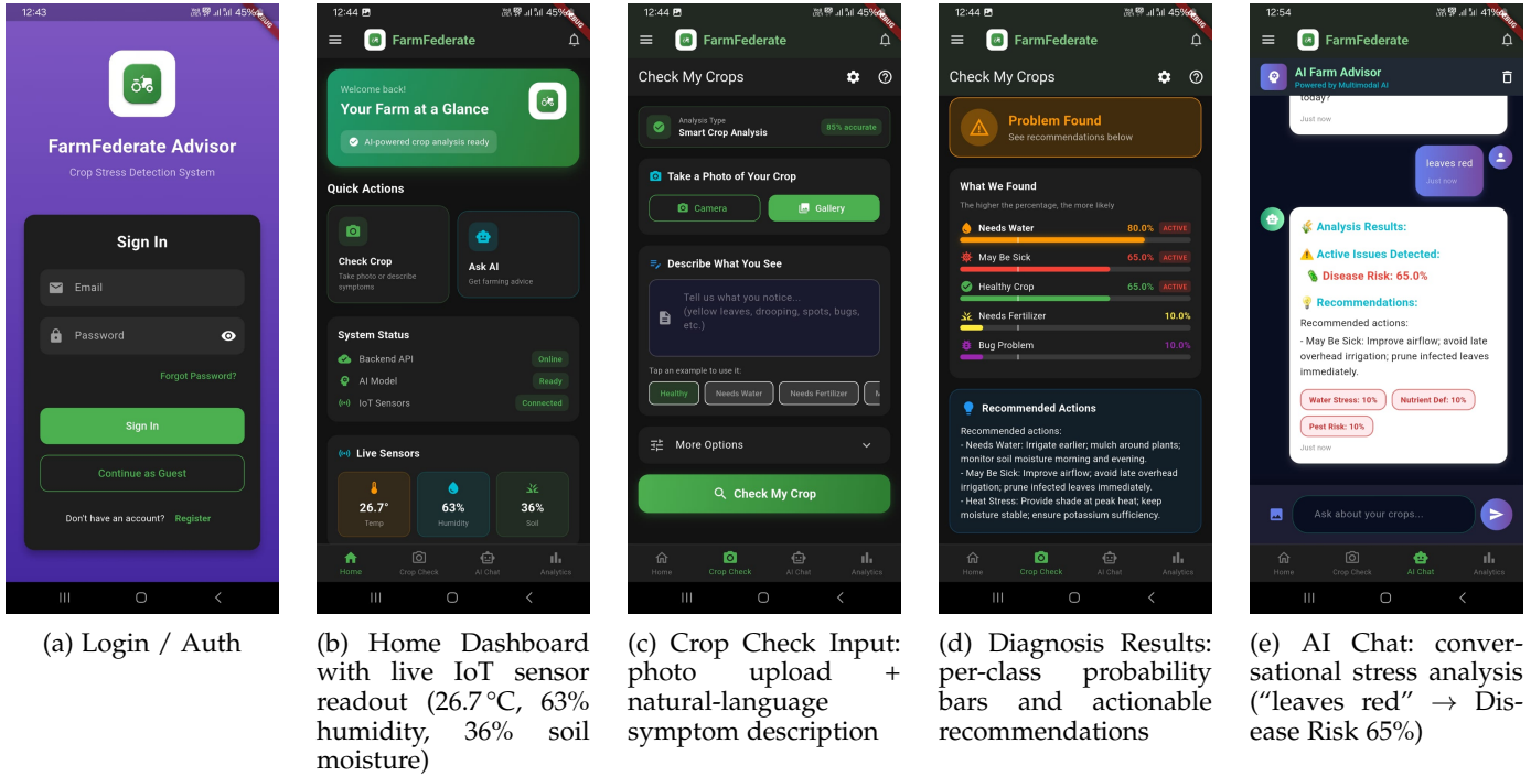
Fig. 25: FarmFederate mobile app — authentication and crop diagnosis screens. The Crop Check screen (c, d) submits image+text to the VLM backend and displays ranked stress probabilities with treatment advice. The AI Chat screen (e) allows conversational diagnosis via the same backend endpoint.
