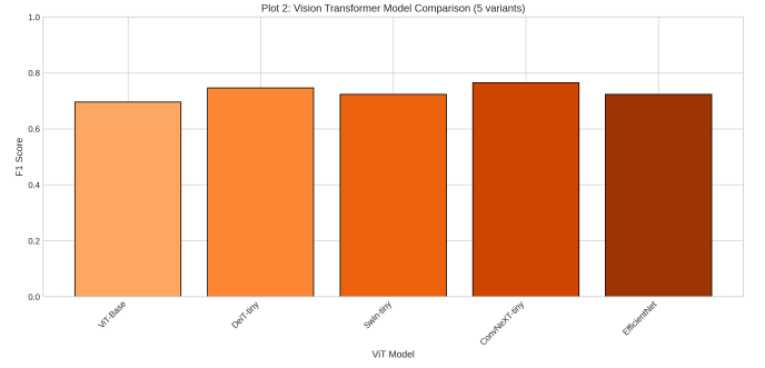
Fig. 7: F1 score comparison across five ViT image encoder variants. ConvNeXT-tiny achieves the highest F1 (0.765), followed by DeiT-tiny (0.747). The performance range (0.70–0.77) demonstrates effective visual feature learning from synthetic crop stress images.
