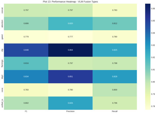
Fig. 9: Performance heatmap across eight VLM fusion architectures showing F1, Precision, and Recall. CLIP and BLIP-2 achieve the highest overall scores, while Gated and CoCa exhibit relatively lower performance.
