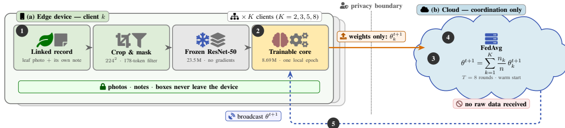
Fig. 7: One FedAvg round: box-linked loading, cropping, masking, and local training of 8.69M parameters remain on the client. The server averages updates; fusion uplink costs 59.5–60.5 MiB per client-round.
