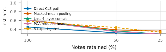
Fig. 3: Text-only accuracy on 75 crops under note deletion; the best rung falls from 0.613 to 0.360. Dashed gates (*) are diagnostic.
