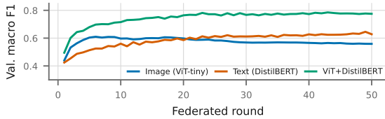
Fig. 14: Rounds against performance for the frozen-encoder systems at \alpha=1 (three seeds \times six client counts). Fusion leads at every round: 0.775 against 0.628 text and 0.559 image.
