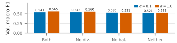
Fig. 12: Anti-collapse arms at both skews, from zero because the finding is that none of them collapses. Values are printed: the arms span 0.044, all of it the balanced sampler, and the diversity term does nothing.
