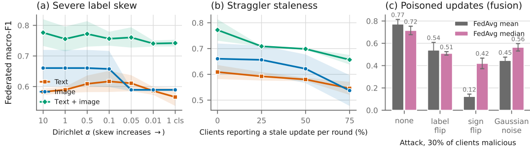
Fig. 16: Federated failure modes on the audited split. (a) Label skew from \alpha=10 to one class per client. (b) Clients reporting an update computed from an earlier global model. (c) Malicious clients under mean against coordinate-wise-median aggregation. Bands are \pm 1 SD over 3 seeds. Client dropout is omitted because it is flat to 70%; the released figure set carries it.
