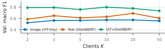
Fig. 15: The same systems against client count. Fusion leads at every count, 0.734–0.799 against 0.587–0.689 for text.
