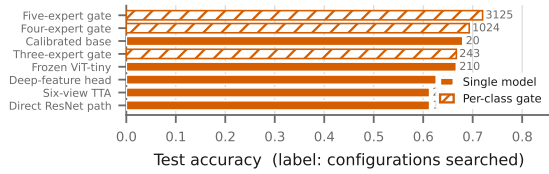
Fig. 5: Alternative image-only systems and search budgets. Accuracy rises from 0.613 to 0.720; hatched class-specific gates are diagnostic, not deployable models.
