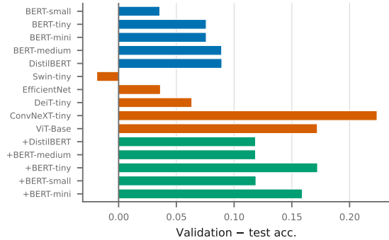
Fig. 6: Validation minus test accuracy per system on the aligned support. A large positive gap is selection that did not transfer from 74 validation crops.
