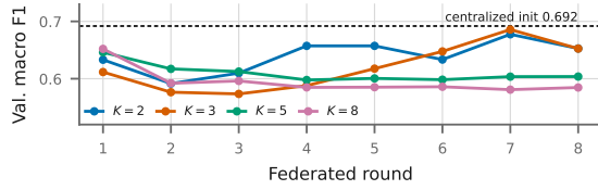
Fig. 9: Rounds against performance for the retained core, one line per client count. Dashed: the centralized initialization each run adapts from. K=2 and 3 climb toward it; K=5 and 8 are flat.
