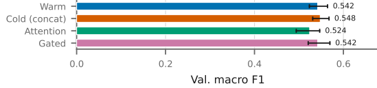
Fig. 13: Every single-architecture matched-setting arm: bars are 3-seed means, whiskers the observed seed range. The cold and concat arms are the same runs. The ranges overlap, so no arm clears the spread.
