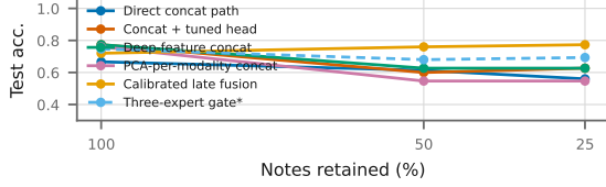
Fig. 4: Fusion under the same deletion: the best rung retains at least 0.760 while text-only falls to 0.360.
