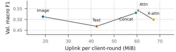
Fig. 11: Uplink cost against accuracy at \alpha=0.1 ; the line orders architectures by uplink rather than interpolating. Cost spans 3.5\times , accuracy 0.073.
