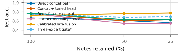
Fig. 4: Text+image rungs under the same deletion. Fusion degrades far more gently: the best rung holds 0.760 or better at every sparsity where the best text rung falls to 0.360.
