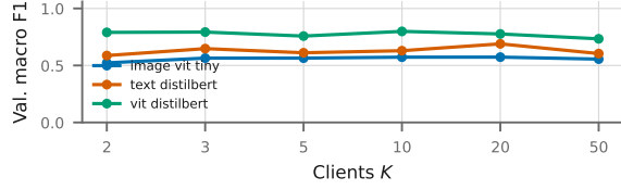
Fig. 2: The same systems against client count. Fusion leads at every count, 0.734–0.799 against 0.587–0.689 for text.
