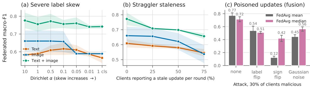
Fig. 8: Federated failure modes on the audited split. (a) Label skew from \alpha=10 to one class per client. (b) Clients reporting an update computed from an earlier global model. (c) Malicious clients under mean against coordinate-wise-median aggregation. Bands are \pm 1 SD over 3 seeds. Client dropout is omitted because it is flat to 70%; the released figure set carries it.
