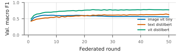
Fig. 9: Per-round convergence at \alpha=1 (three seeds \times six client counts). Fusion leads at every round: 0.775 against 0.628 text, 0.559 image.
