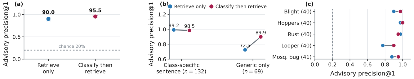
Fig. 7: Measured Classify–Retrieve–Advise quality on the templated symptom corpus: 472 passages, 201 queries, exact inner-product search. (a) Precision@1 with bootstrap intervals against chance; (b) split by whether the query holds a class-unique sentence; (c) per class. Same five classes as the diagnostic experiments, but a different corpus and support, never pooled with them.
